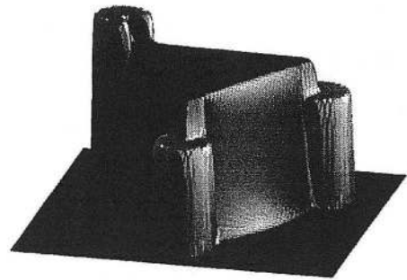
Figure 7: A strongly off center fixation point: on the left equispaced contour lines of the point-of-view surface are shown and on the right the subjective surface is visualized.
