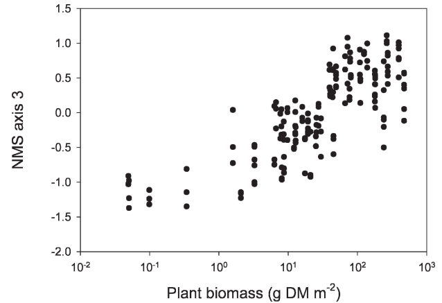
Fig. 8. Relationship between the third NMS ordination axis for epiphytic samples and plant biomass ( r^2 = 0.63 , p < 0.0001 ).
