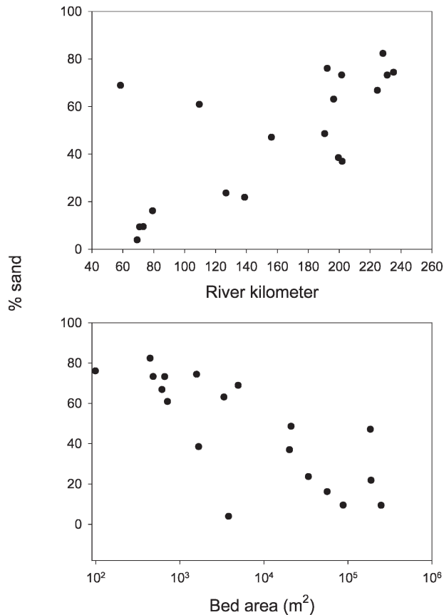
Fig. 1. Sediment texture as a function of position along the river and size of the macrophyte bed (which is scaled logarithmically). For the upper panel, r^2 = 0.48 , p = 0.001 ; for the lower panel, r^2 = 0.49 , p = 0.004 .
