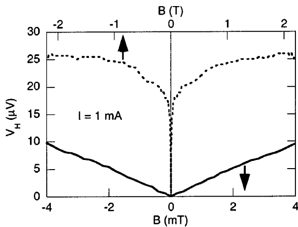
FIG. 5. Hall voltage as a function of the in-plane magnetic induction. Only a few devices show this behavior.
