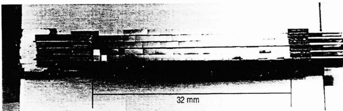
Figure 9. Test assembly of a 5x32 array of 1 mm 2 , 1µm thick PUD mechanical models. The detector model shown is identical in geometry to that whose electrical NEP was measured to be 3 \times 10^{-18} W/√Hz at 85mK.
