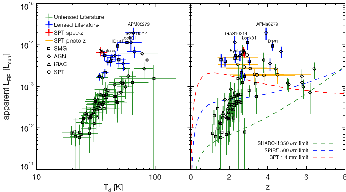
Figure 3. Left: apparent L_{\text{FIR}} vs. T_d for all unlensed (green symbols) and lensed (blue symbols) 350 \mu\text{m} detected SMGs and AGNs (squares and diamonds, respectively) with spectroscopic redshifts at z > 1 (see Section 3.3 for references). Apparent (i.e., lensed) FIR luminosities vs. dust temperature for the two SPT sources with spectroscopic redshifts presented in this paper (red symbols). For all sources, the FIR luminosities and dust temperatures were derived by fitting a modified blackbody law with \beta = 2.0 becoming optically thick at \lambda_c < 100 \mu\text{m} . Right: the FIR luminosity as a function of redshift for the same sources. The nine SPT sources presented here that lack spectroscopic redshifts are also plotted (black dots with yellow error bars) with their photometric redshift estimates and associated uncertainties. The uncertainty on L_{\text{FIR}} given the assumed photometric redshift is described in Section 3.3, which assumes T_d = 34 \text{ K} —the median dust temperature of the unlensed population. The green, blue, and red dashed curves show the limiting FIR luminosity as a function of redshift corresponding to the effective SHARC-II 350 \mu\text{m} survey limit (rms \sim 5 \text{ mJy} ), three times the SPIRE 500 \mu\text{m} confusion limit (30 mJy), and the 3\sigma SPT 2.0 \text{ mm} survey limit (3.9 mJy), respectively, given the SED model of this paper and assuming a 35 K dust temperature. The SPT survey, with its longer wavelength selection, is more sensitive to sources at the highest redshifts ( z > 5 ) than Herschel , and the large survey area of SPT makes it sensitive to sources that are among the most rare and most highly magnified.
