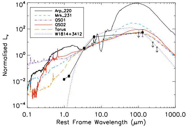
Figure 6. SED of W1814+3412 at z=2.452 , including the 850 \mu\text{m} SCUBA-2 data with Polletta galaxy templates Arp 220, Mrk 231, QSO 1, QSO 2 and torus (Polletta et al. 2007) and W1814+3412 template (Blain et al. in prep.) normalized at rest-frame 3 \mu\text{m} . CSO SHARC-II 350 \mu\text{m} and 450 \mu\text{m} and CSO Bolocam 1100 \mu\text{m} data points from Wu et al. (2012) are included. Detections are represented by filled circles, while 2\sigma upper limits are represented by arrows.
