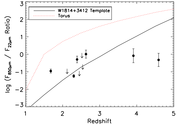
Figure 7. The submm to mid-IR ratio ( F_{850\mu\text{m}}/F_{22\mu\text{m}} ) of the 10 Hot DOGs. The solid line shows the W1814+3412 template (Blain et al., in preparation) and the dotted line shows Polletta torus template (Polletta et al. 2007) as a function of redshift. Detections are represented by filled circles, while 2\sigma upper limits are represented by arrows.
