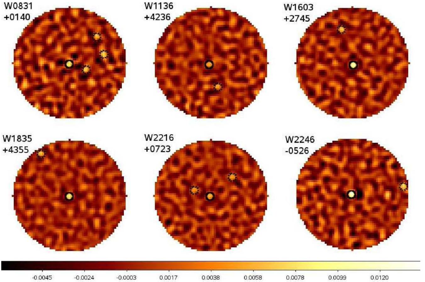
Figure 1. SCUBA-2 850 \mu\text{m} 1.5-arcmin-radius maps of the six detected targets; W0831+0140, W1136+4236, W1603+2745, W1835+4355, W2216+0723 and W2246–0526. The solid circles show the 15-arcmin beam-sized apertures centred on the WISE RA Dec. of the targets. Serendipitous sources brighter than 3\sigma and within 1.5-arcmin-radius of the WISE target are shown by the dotted 15-arcmin beam-sized circles. The colour flux bar at the bottom is in Jy. North is up, east is to the left.
