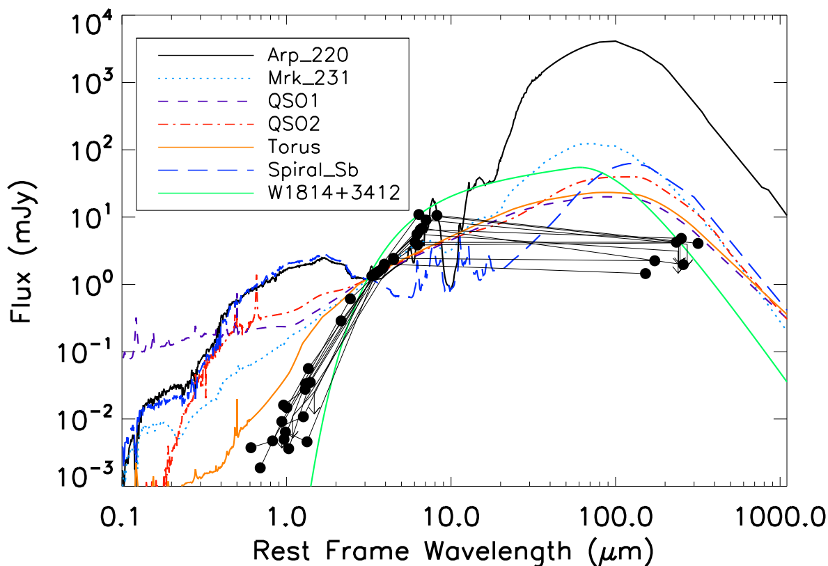
Figure 5. SEDs of the 10 Hot DOGs including the 850 \mu\text{m} SCUBA-2 data in rest-frame wavelengths with Arp 220, Mrk 231, QSO 1, QSO 2 and torus galaxy templates from Polletta et al. (2007) and W1814+3412 template from Blain et al. (in prep.) normalized at 3 \mu\text{m} . Detections are represented by filled circles, while 2\sigma upper limits are represented by arrows. The data points for the Hot DOGs are connected for clarity, and do not represent the true SED.
