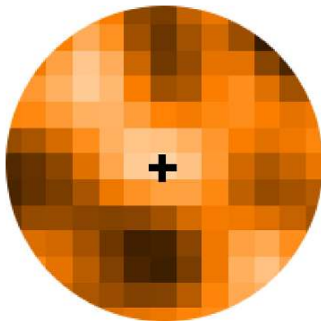
Figure 4. SCUBA-2 850 \mu\text{m} 48 arcsec radius map showing the central region of the four undetected targets stacked together. The cross shows the central pixel. North is up, east is to the left.
