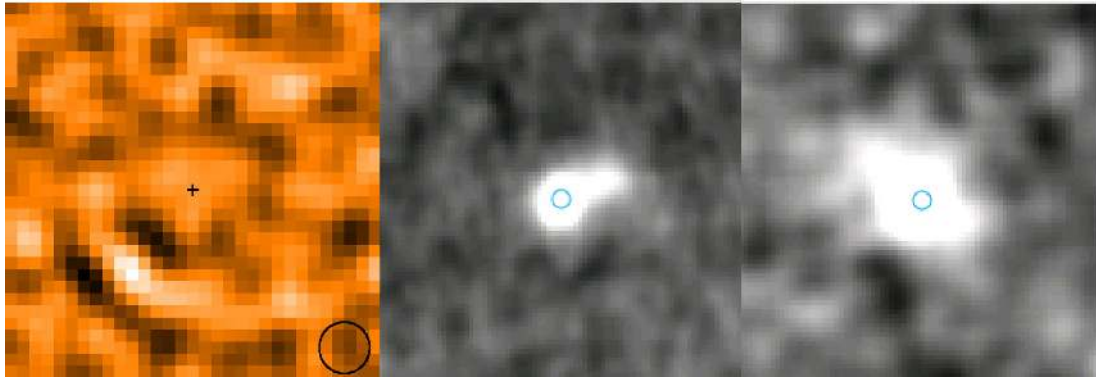
Figure 3. Left: the 2 \times 2 arcmin 2 SCUBA-2 850 \mu\text{m} map of W2026+0716. Increasing the aperture size out to 29 arcsec in diameter increases the measured flux for this target, which could be due to multiple components of the target or to nearby, unrelated sources. The beam size (15 arcsec diameter) is represented by the black circle. Note the 4.4\sigma serendipitous source \sim 35 arcsec south-east of the target. Centre and right: WISE W3 and W4 images, respectively, showing the same region of sky, with a circle showing the WISE determined position of the target. The target is not extended in the WISE images. North is up, and east is to the left.
