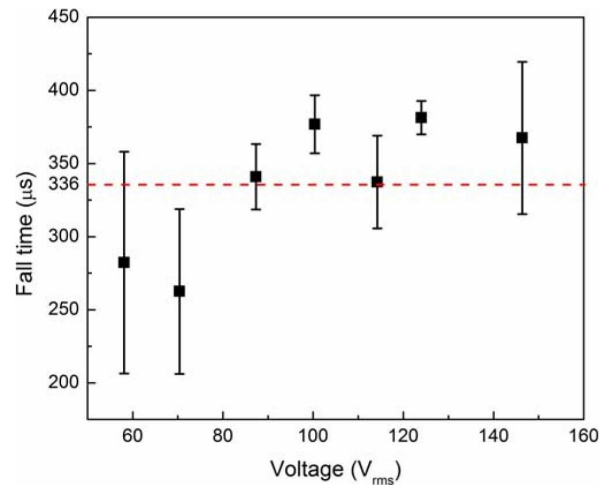
Fig. 4. Measured decay time of the PS-BPLC cell from each gray level to T0. Black solid squares are the measured results and dashed red lines stand for average fall time, which is 335.5 \mu\text{s} .
