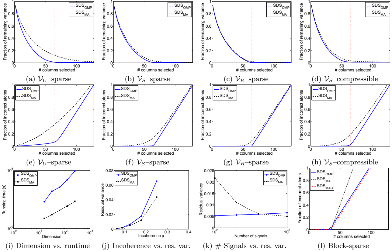
Figure 2. Results of 50 trials: (a-c) Variance reduction achieved by SDS OMP and SDS MA on the collections \mathcal{V}_{U,S,R} for 5-sparse signals in 64 dimensions. (e-g) Percentage of incorrectly selected columns on the same collections. (d) Variance reduction for compressible signals in 64 dimensions for \mathcal{V}_S . (h) Corresponding column selection performance. (i) SDS MA is orders of magnitude faster than SDS OMP over a broad range of dimensions. (j) As incoherence decreases, the algorithm effectiveness in variance reduction improve. (k) The variance reduction performance of SDS MA improves with the number of training samples. (l) Exploiting block-sparse structure in signals leads to improved dictionary selection performance.
