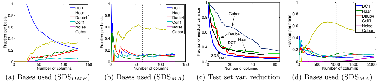
Figure 3. Experiments on natural image patches. (a,b,c) Fractions of bases selected for SDS_{OMP} and SDS_{MA} with d = 64 (a,b), and the corresponding variance reduction on test patches. (d) Fractions of bases selected for SDS_{MA} with d = 1024 .
