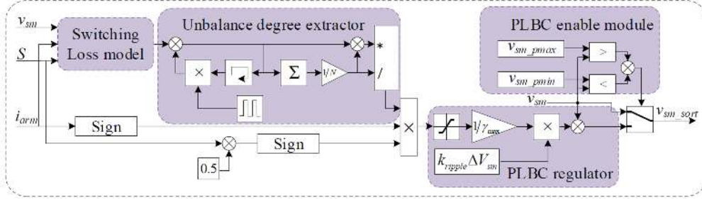
Fig. 4. Submodule level power loss balancing control scheme.
