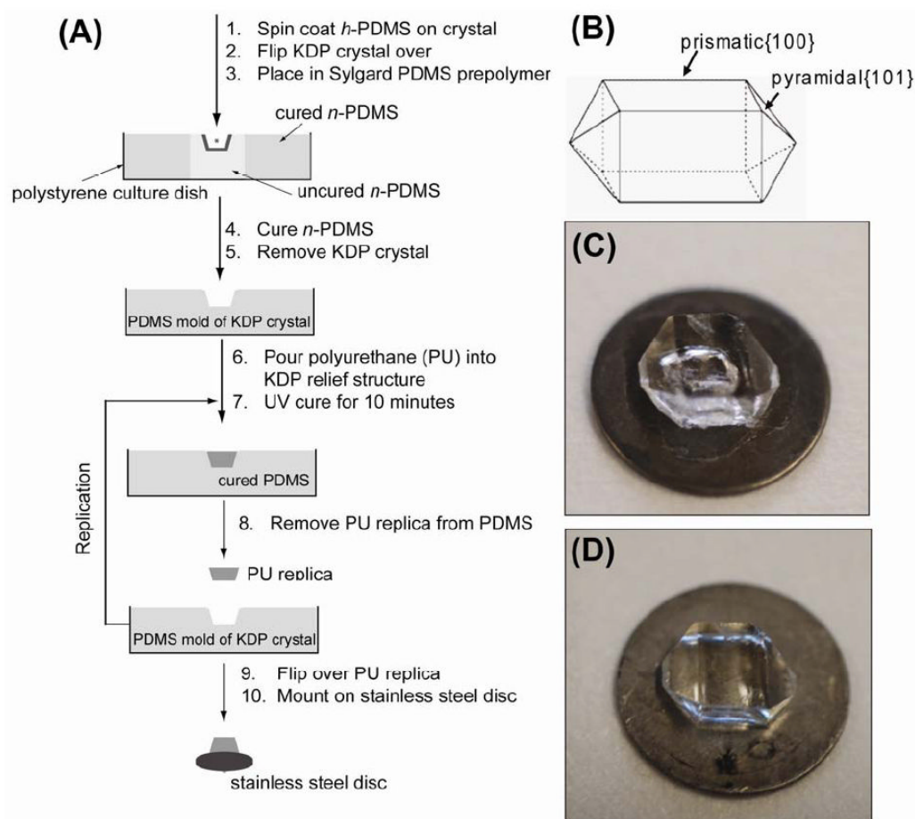
Figure 2. (A) Schematic of the replication procedure of a crystal surface on the {100} and {101} oriented surfaces of KDP using a PDMS mold and PU replica. (B) Schematic of macroscopic KDP crystal showing location of the {100} and {101} faces. The elementary and macro-steps replicated on the KDP surface are located on the {100} face. (C) Photograph of the original KDP crystal supported on a stainless steel disk (15-mm diameter). The hole seen in the image is on the underside of the crystal and represents the original location of the seed crystal used during crystal growth. (D) A PU replica of the original crystal in (C) supported on a stainless steel disk. The hole of the seed crystal is now missing from the PU replica because the {100} and {101} surfaces are replicated in part (A). (Only the {100} surface was subsequently imaged due to geometric constraints.) The same procedure was used to replicate the surface of calcite{104}.
