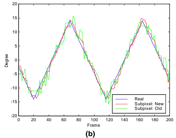
Figure 7. Azimuth angle tracking result of a sequence segment.
