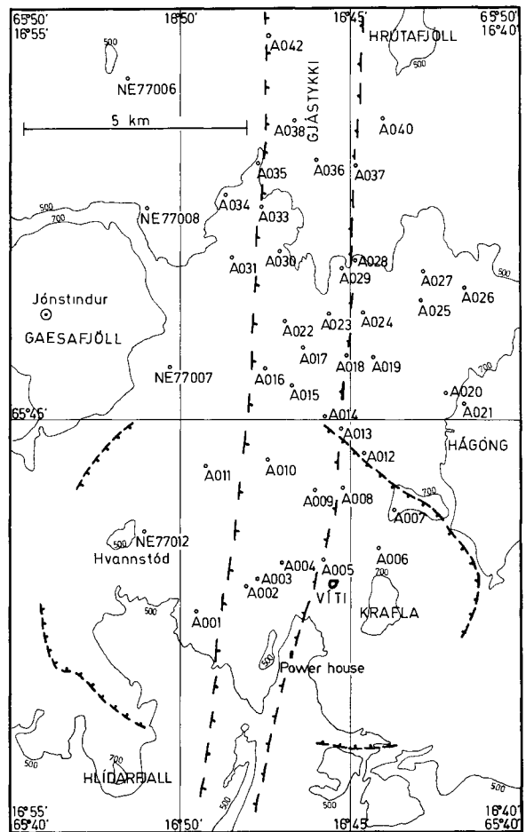
Fig. 2. Location of the stations used in distance measurements with geodimeter in the Krafla-Gjástykki area
