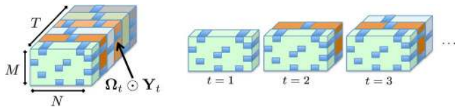
Fig. 2. Tensor data with missing entries. (Left) Batch data, and slice \Omega_t \circ \mathbf{Y}_t along the time (tube) dimension. (Right) Streaming data, where slices \Omega_t \circ \mathbf{Y}_t become available for t = 1, 2, \dots
