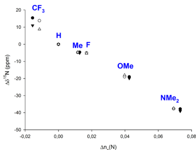
Figure 2. ^{15}\text{N} NMR chemical shift changes (relative to 1a or 2a , respectively), \Delta\delta^{15}\text{N} , of substituted pyridines (●), of the corresponding 1,2-bis((pyridine-2-ylethynyl)benzene) ligands 3a–f (○), and of their [\text{N}\cdots\text{I}\cdots\text{N}]^+ complexes, 1a–d,f (▼) and 2a–f (△), respectively, strongly correlate to the corresponding changes in the \pi(\text{N}) orbital population. This indicates that the variation in \delta^{15}\text{N} is dominantly governed by the paramagnetic ring currents in the pyridine moieties.
