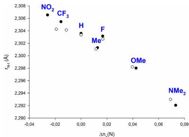
Figure 3. Correlation of the N–I bond distance with the change in the \pi(\text{N}) population of iodine(I) complexes of substituted pyridines ( 1a–g ) (●) and of the corresponding 1,2-bis((pyridine-2-ylethynyl)-benzene) ligands ( 2a–g ) (○).
