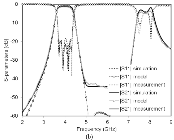
Fig. 11. Four-pole filter based on a quarter-mode SIW cavity (from [18]): (a) Photograph of the prototype; (b) Comparison between simulated and measured scattering parameters of the filter.
