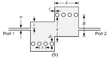
Fig. 10. Coupling mechanisms in a two-pole filter based on quarter-mode SIW cavity (from [18]): (a) Coupling is obtained by removing the common posts; (b) Coupling is controlled by shifting the two cavities.
