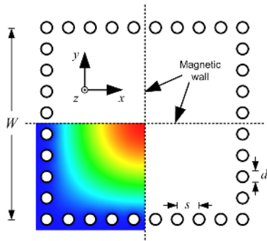
Fig. 9. Geometry of a quarter-mode SIW cavity and representation of the electric field of the fundamental mode (from [18]).
