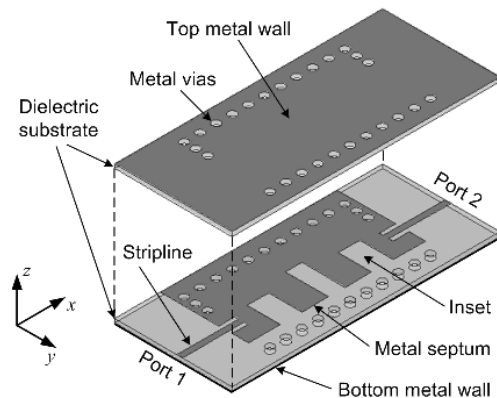
Fig. 3. Geometry of a filter based on the folded SIW cavity (from [16]).
