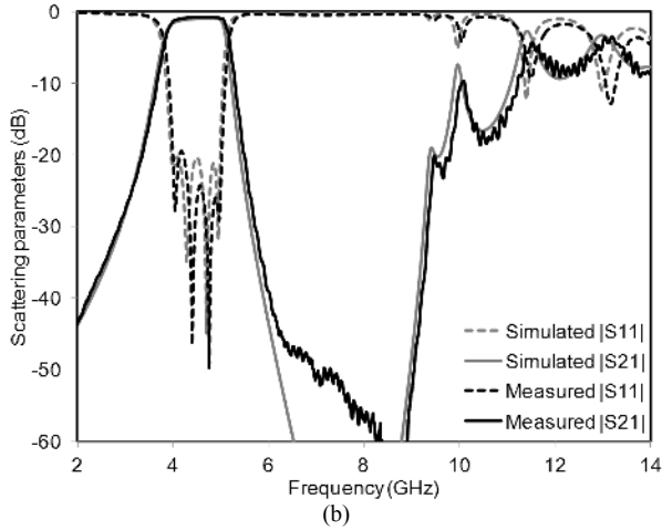
Fig. 8. Four-pole filter based on a half-mode SIW cavity (from [17]): (a) Photograph of the prototype; (b) Comparison between simulated and measured scattering parameters of the filter.
