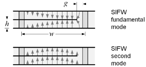
Fig. 2. Geometry of a folded SIW and representation of the electric field of the first two modes.
