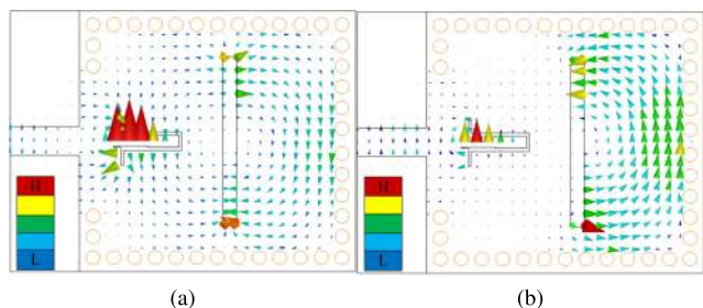
FIGURE 5. The distribution of H-field. (b) TE_{120} mode (a) hybrid mode.
