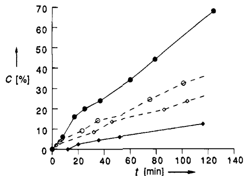
Figure 3. Isomerization of 4-allylcatechol (○) and allylbenzene (◇) by compound 5 (solid lines and filled marks) and by \text{HRh}(\text{CO})[\text{P}(\text{O}i\text{Pr})_3]_3 (dotted lines and open marks). Conditions: [\text{Rh}] = [\text{substrate}] \approx 17 \text{ mM} , T = 25^\circ\text{C} , solvent chloroform.
