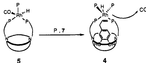
Figure 4. Substrate-induced formation of complex 4 from complex 5 .
