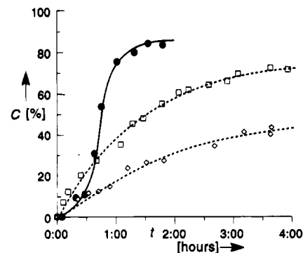
Figure 7. Effect of resorcinol (●) on the hydrogenation of 7 by compound 4 . For comparison also the blank reactions without any additives are shown: 7 and HRh[P(OPh) 3 ] 4 (◇); 7 and 4 (□). Conditions: [Rh] = 5.4 mM, T = 25.0 \pm 0.1 °C, 1 additional equiv of P(OPh) 3 , solvent chloroform.
