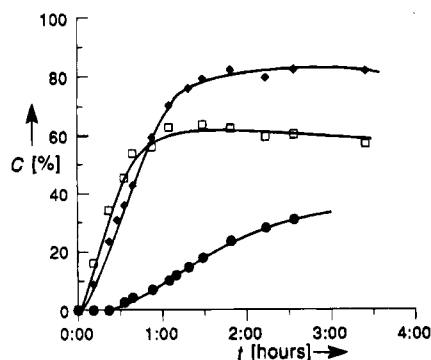
Figure 6. Competitive hydrogenation of 6 (●), 7 (◆), and 8 (□) by compound 4 . Conditions: [Rh] = 5.4 mM, [substrate]/[Rh] = 3, T = 25.0 \pm 0.1 °C, 1 additional equiv of P(OPh) 3 , solvent chloroform.
