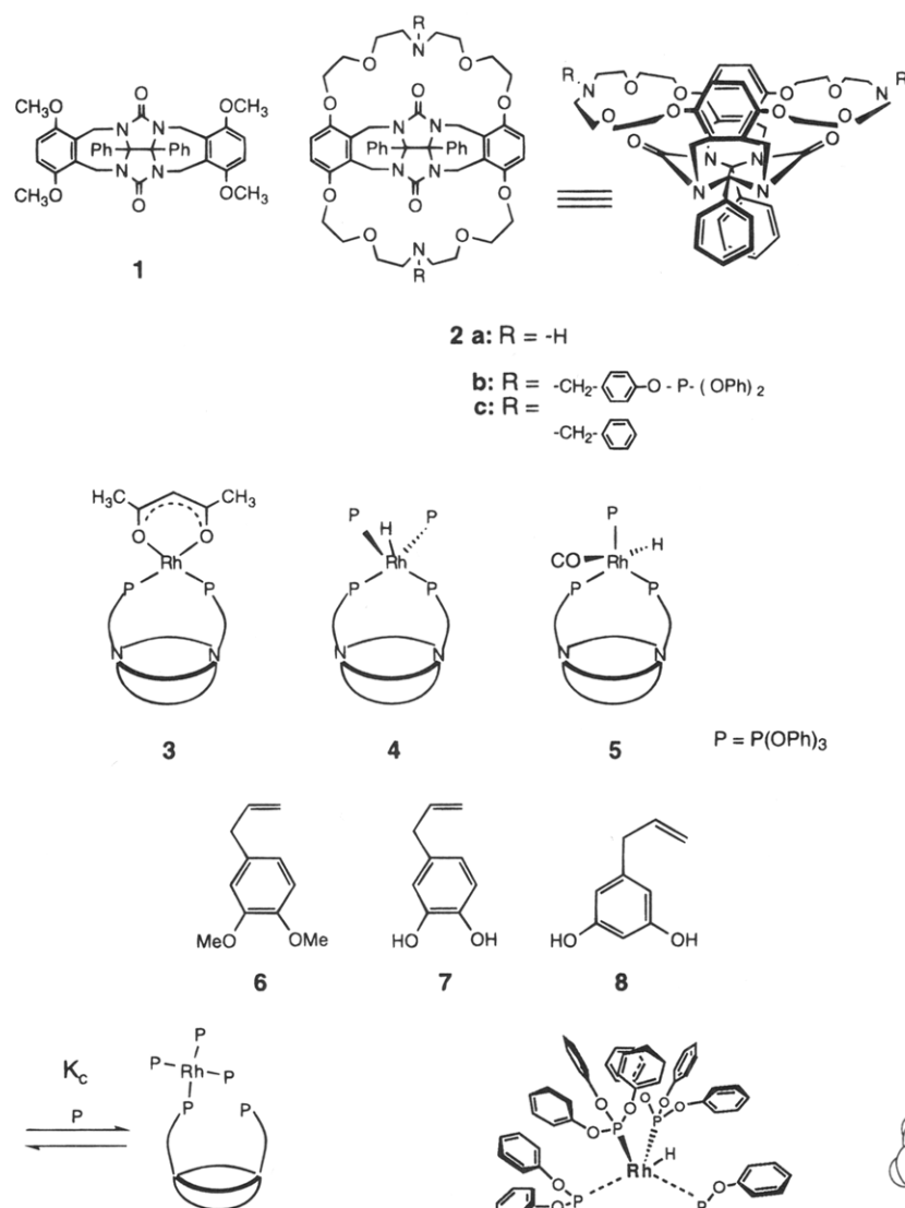
Figure 1. Interconversion equilibrium between the chelated form of compound 4 and a form in which one of the ligands of the receptor molecule is replaced by a \text{P}(\text{OPh})_3 ligand.
