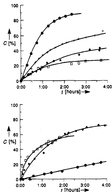
Figure 5. Hydrogenation of 6 (●), eugenol (+), 7 (◇), and 8 (□) by \text{HRh}[\text{P}(\text{OPh})_3]_4 (top) and compound 4 (bottom). Conditions: [\text{Rh}] = 5.4 \text{ mM} , T = 25.0 \pm 0.1 \text{ }^\circ\text{C} , 1 additional equiv of \text{P}(\text{OPh})_3 , solvent chloroform.
