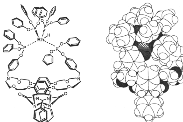
Figure 2. Drawing and computer-generated structure of compound 4.
