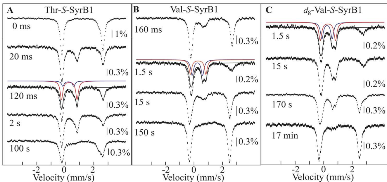
Figure 2. 4.2-K/0-mT Mössbauer spectra of selected samples prepared by reacting the SyrB2• Fe(II) • Cl•αKG• substrate complex at 5 °C with Q-saturated buffer. Substrates and reaction times are indicated. The final sample compositions are given in Materials and Methods. Solid lines are simulations of the spectra of the two Fe(IV) components of the chloroferryl state (red and blue) and the summation of their contributions (black). The isomer shift and quadrupole splitting parameters of the Fe(IV) intermediate(s) are as follows: L -Thr, \delta_1=0.30 mm/s, \Delta E_{Q,1}=1.09 mm/s and \delta_2=0.23 mm/s, \Delta E_{Q,2}=0.76 mm/s; L -Val and d 8 - L -Val, \delta_1=0.29 mm/s, \Delta E_{Q,1}=1.09 mm/s and \delta_2=0.24 mm/s, \Delta E_{Q,2}=0.73 mm/s.
