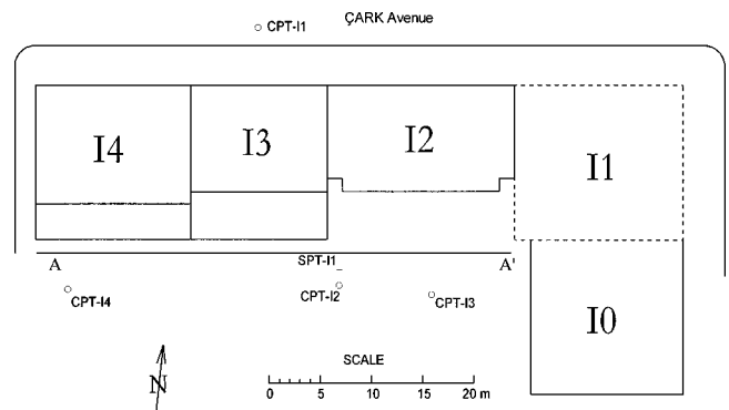
Fig. 11. Plan view of Site I and location of subsurface exploration points
