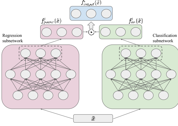
Figure 2: A generic subtask gated network.
