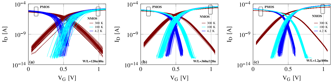
FIGURE 5. I_D - V_G curves for a single die (48 devices per geometry) at T = 300 K, 100 K and 4.2 K: (a) W/L=120n/40n ; (b) W/L=360n/120n and (c) W/L=1.2\mu/400n . |V_{DS}| = 50 mV. V_S = 0 V for NMOS and 1.1 V for PMOS, respectively.
