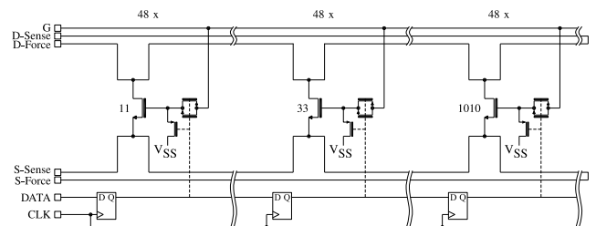
FIGURE 3. Simplified schematic of the NMOS mismatch characterization array of chip #1.
