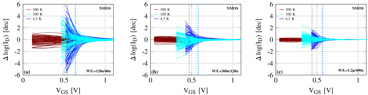
FIGURE 7. NMOS drain-current mismatch of 72 device pairs (3 dies) at T = 300 K, 100 K and 4.2 K: (a) W/L=120n/40n ; (b) W/L=360n/120n and (c) W/L=1.2\mu/400n . V_{TH} marked by dashed lines. V_{DS} = 50 mV.
