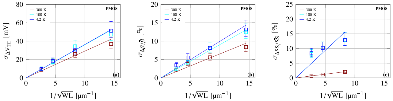
FIGURE 8. Pelgrom plots of PMOS with L=40\text{nm} device length at T = 300\text{K} , 100\text{K} and 4.2\text{K} for: (a) \sigma_{\Delta V_{TH}} ; (b) \sigma_{\Delta\beta/\beta} and (c) \sigma_{\Delta SS/SS} . 95% confidence intervals are shown.
