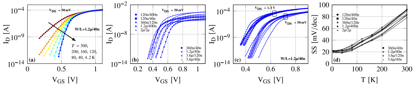
FIGURE 6. NMOS device behaviour over temperature: (a) I_D - V_G curves of a W/L=1.2\mu/40n device; (b) I_D - V_G curves of all 9 geometries at T = 4.2 K; (c) I_D - V_G curves of 10 W/L=1.2\mu/40n devices at T = 4.2 K and (d) extracted SS ( V_{DS} = 50 mV) as function of temperature for all 9 geometries.
