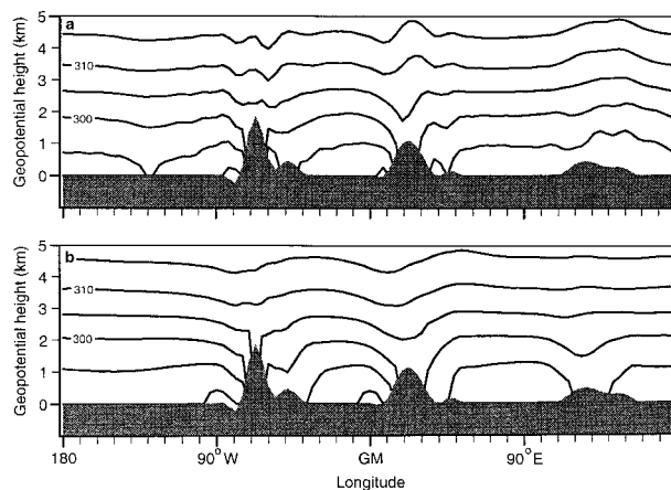
FIG. 13. Longitude–height plots at 24°S showing isentropes in winter (Jun–Aug): (a) from ECMWF analyses for 1983–88 and (b) from day 15 of a model simulation with a Jun–Aug initial state from the same analyses and forced with mountains only. The terrain profile at 24°S is also shown. The contour interval is 5 K.
