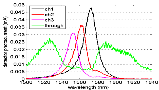
Figure 4: Spectral response (photocurrent, linear scale) of the three rightmost channels and the through detector. Channel 4 was damaged.
