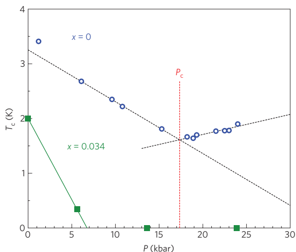
Figure 4 | Effect of impurity scattering on T_c in \text{KFe}_2\text{As}_2 . Pressure dependence of T_c in \text{KFe}_2\text{As}_2 for a nominally pure sample (open circles, sample B) and a sample with 3.4% Co impurities (filled squares, \text{K}(\text{Fe}_{1-x}\text{Co}_x)_2\text{As}_2 with x = 0.034 , from resistivity data in Supplementary Fig. S3). The dotted lines are linear fits to the pure data within 10 kbar on either side of P_c . The solid green line is a linear fit to the first two data points of the impure sample. Note how T_c is suppressed by the addition of impurities both below and above P_c , showing that the pairing states on both sides of the transition are highly sensitive to impurity scattering.
