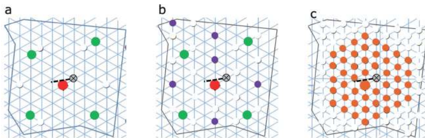
Figure 4 A notional stepwise development plan for a seismic monitoring network and alternative SET buried net. The resource is assumed to be at a depth of ~1.5-2 km, the target area to be monitored ~ 5 x 5 km, and the exploration/lease area equal to be ~ 10 x 10 km. A well with a ~1 km long lateral has been planned as shown by the grey circle. A dense face-centered hexagonal station grid was used so a densified SET buried array could easily be accommodated. (a) Step 1 event detection – red circle: the initial seismicity-detection station, preferably as deep as possible in a borehole. Step 2 event location – green circles: four additional borehole stations. (b) Step 3 tomography – purple circles. (c) A SET buried array – orange circles: an alternative monitoring development strategy, comprised of a ~48 stations in 100 m deep boreholes, a density of ~2 stations/km 2 .
