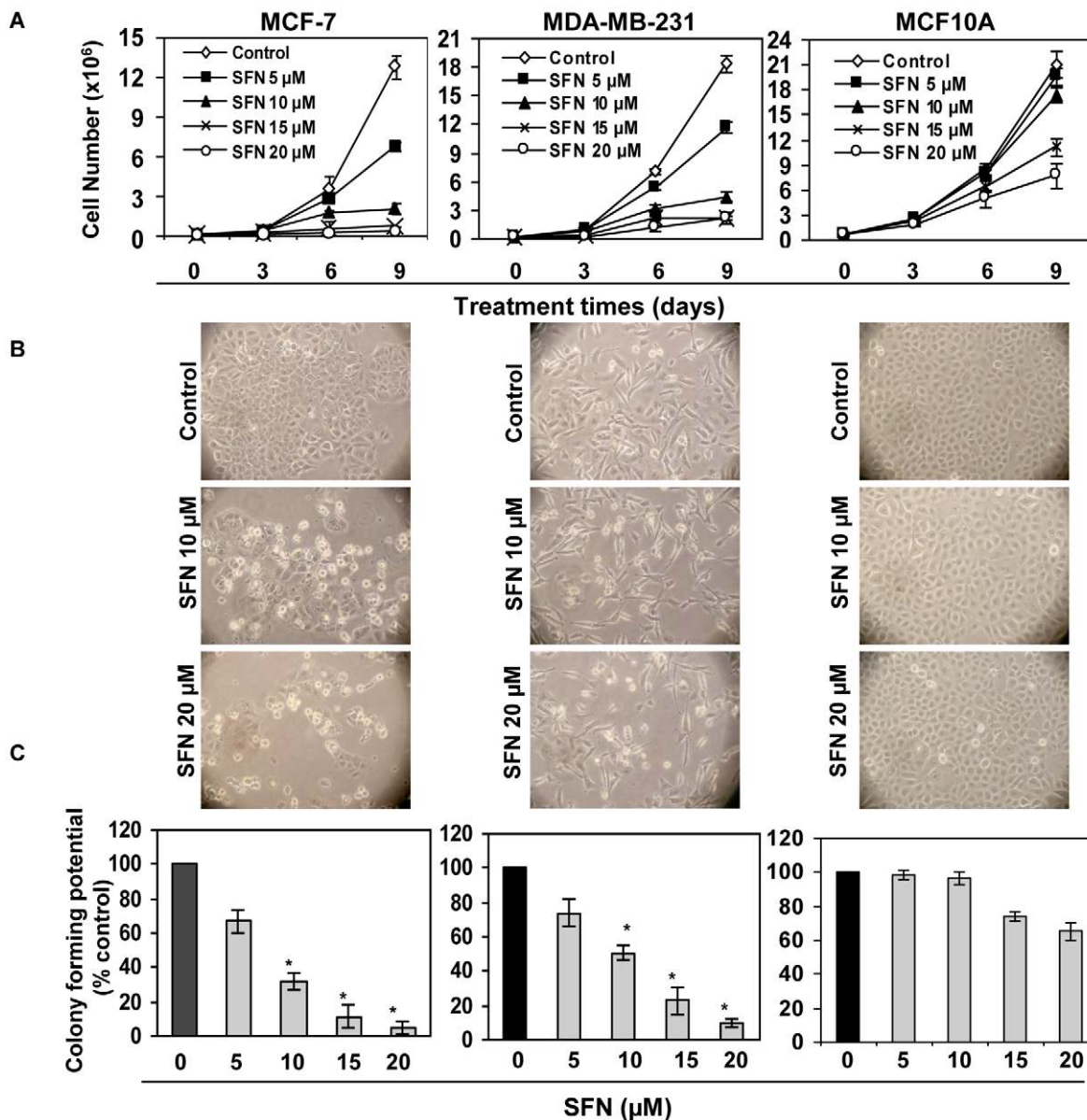
Figure 1. SFN inhibits proliferation of breast cancer cells but has negligible effect on control MCF10A cells up to 10 \mu M SFN. A) Breast cancer MCF-7 (left panel) and MDA-MB-231 (middle panel) cells as well as control MCF10A cells (right panel) were treated with SFN (0–20 \mu M) for 3, 6 and 9 days. Growth curve kinetics was obtained by counting the total number of viable cells at the indicated time intervals using trypan blue staining. Results were obtained from three independent experiments, mean \pm SD. B) Morphological changes with SFN treatment on MCF-7 (left panel), MDA-MB-231 (middle panel) and MCF10A (right panel) cells. The white floating cells are indicative of apoptotic/dead cells. View, X100. C) Treatment with SFN (0–20 \mu M) inhibits the proliferation potential of human breast cancer MCF-7 (left panel) and MDA-MB-231 (middle panel) cells in a dose-dependent manner. Control MCF10A cells (right panel) did not show a significant inhibition of colony forming potential at lower doses of SFN. Proliferation of cells was assayed by the colonogenic assay. Colonies were stained using trypan blue and the total number counted at the end of the 15-day period protocol. The experiment was repeated three times and each point indicates the mean \pm SD of the number of colonies formed. * P < 0.05 . doi:10.1371/journal.pone.0011457.g001
