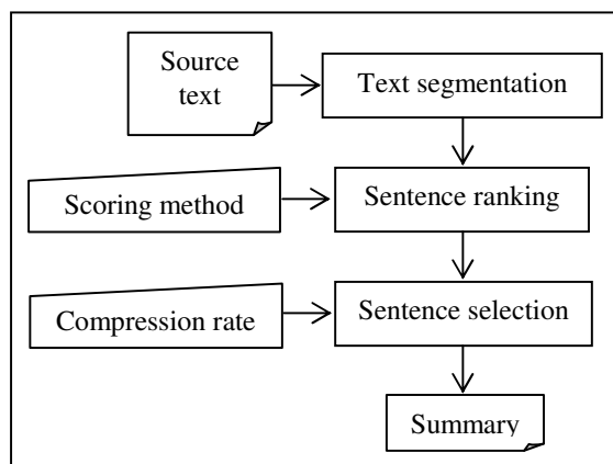
Figure 1. GistSumm architecture
