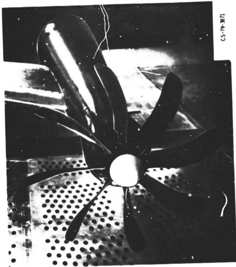
Figure 9. - The SRI propeller configuration in the NASA-Lewis Research Center 8- by 6-Foot Wind Tunnel.
