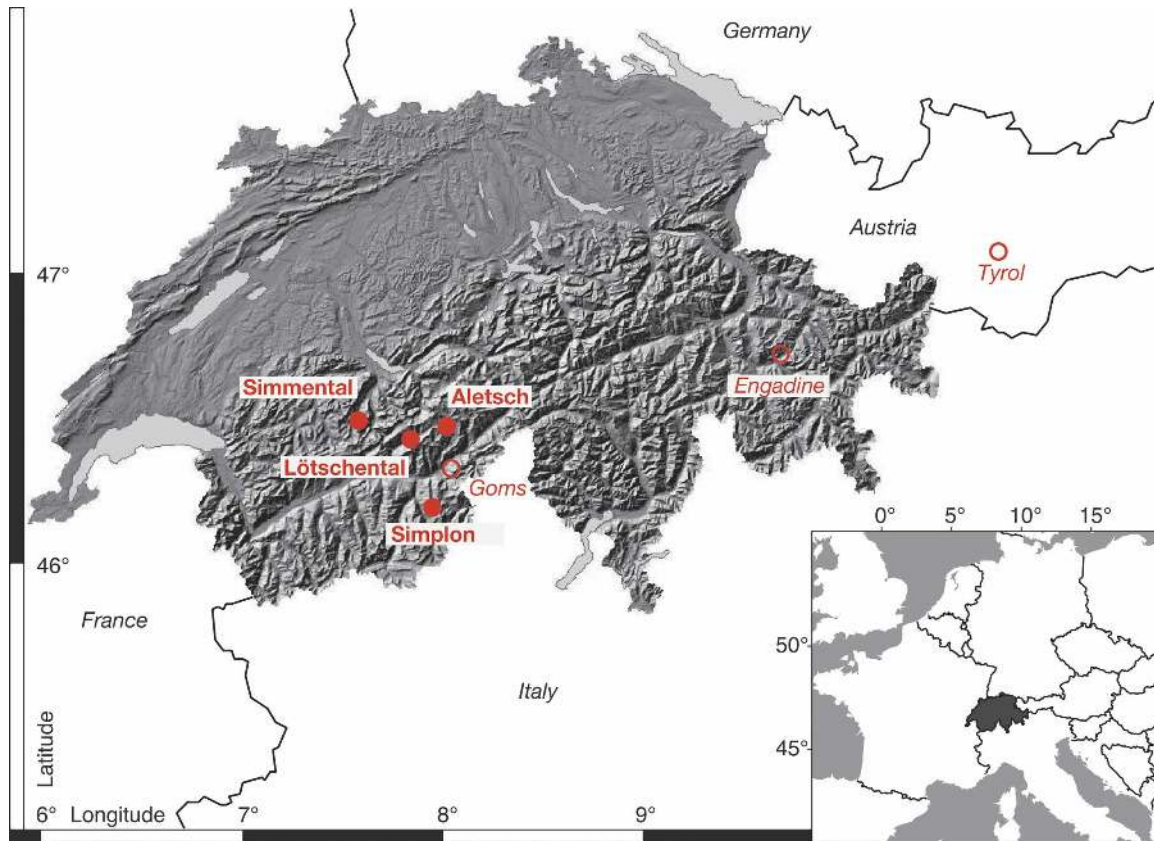
FIG. 1. Location of the four MXD tree-ring sites (red dots, bold) within the Swiss Alps, and the additional Alpine RW sites (red circles, italic) used by Büntgen et al. (2005a).
