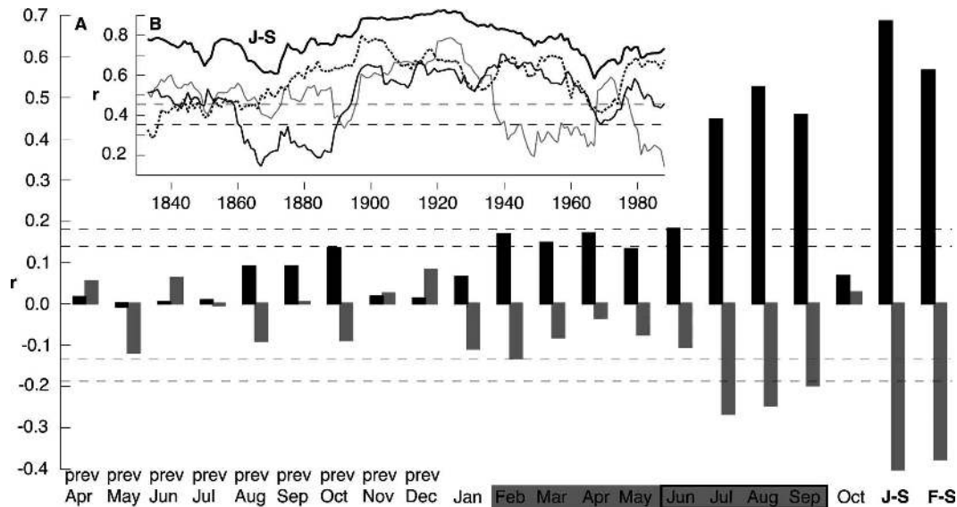
FIG. 3. Climate response of the RCS-MXD chronology. (a) Correlations with high-elevation monthly mean temperatures (black) and precipitation (gray) of the previous and current year (1818–2003). [(b), inset to a] Moving 31-yr correlations with current-year July (black), August (dashed), September (gray), and JJAS (black bold, labeled J-S) mean temperatures. Horizontal lines denote 95% and 99% significance levels, corrected for lag-1 autocorrelation (Trenberth 1984) using the month with the highest autocorrelation.
