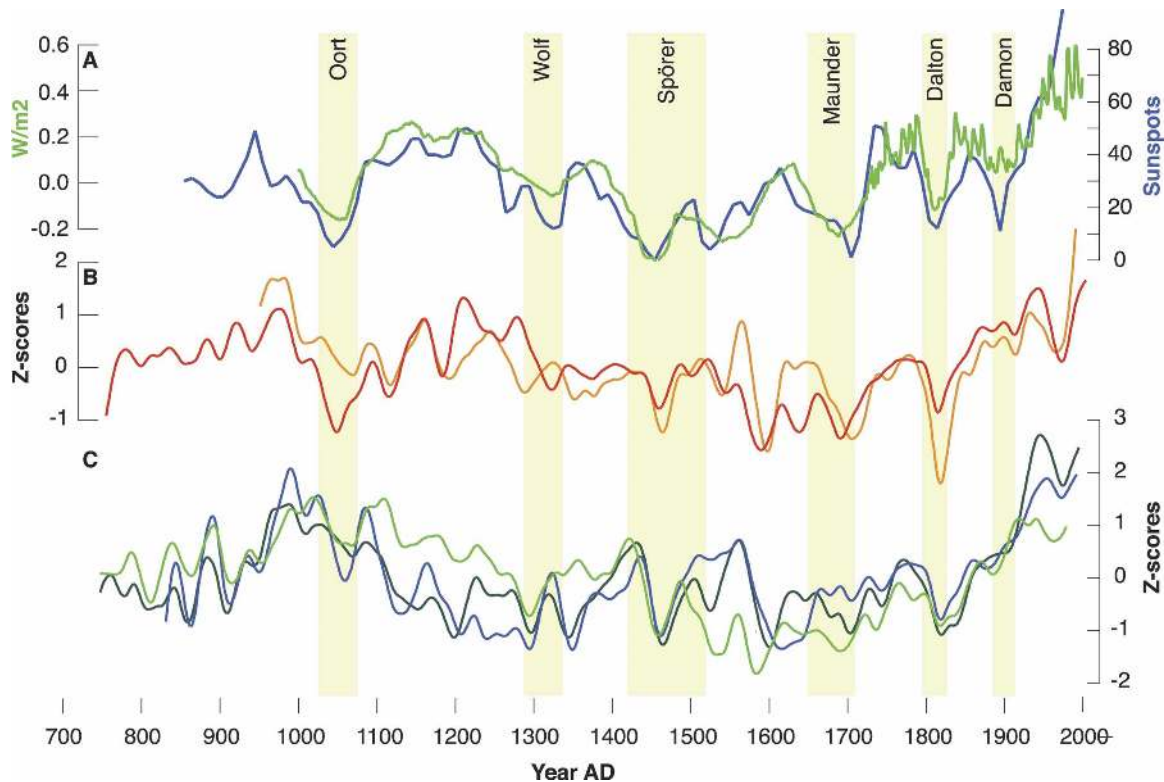
FIG. 7. (a) Low-frequency estimates of solar activity (green; Crowley 2000) and sunspot numbers (blue; Usoskin et al. 2003). (b) The MXD-based Alpine temperature reconstructions (red; this study) and RW-based reconstruction (orange; Büntgen et al. 2005a). (c) Large-scale temperature reconstructions (blue: Esper et al. 2002, green: Moberg et al. 2005, and dark green: D'Arrigo et al. 2006). All temperature reconstructions were transformed to z scores over the 951–1979 common period and were 40-yr low-pass filtered. Shadings denote the timing of great solar minima (Stuiver and Braziunas 1989). The sunspot number reconstruction (11-yr smoothed) is not independent of the spliced solar activity reconstruction, since both are based on ice core measurements of ^{10}\text{Be} cosmogenic isotopes (Bard et al. 2000; Beer et al. 2000).
