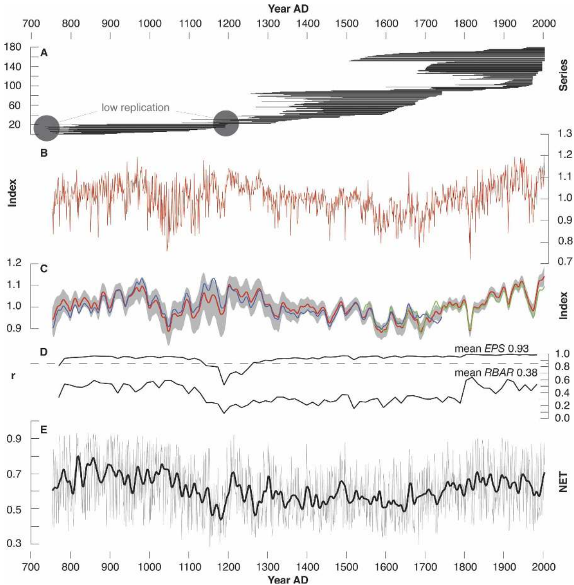
FIG. 2. The Alpine RCS-MXD chronology. (a) Temporal distribution of the 180 MXD samples. (b) The RCS-MXD chronology (red), and (c) the RCS-MXD chronology (red) with 95% bootstrap confidence limits (gray), and RCS chronologies after recent/historic data splitting (green/blue), all 20-yr low-pass filtered. (d) The temporal signal strength of the chronology is shown by EPS and RBAR statistics, with the horizontal line indicating the 0.85 EPS validity threshold, and (e) the 1 - \text{NET} parameter with high values indicating internal signal strength. The black line derives from 20-yr low-pass filtering, with both ends padded using the mean of the last 10 yr, somewhat comparable to the method described by Mann (2004).
