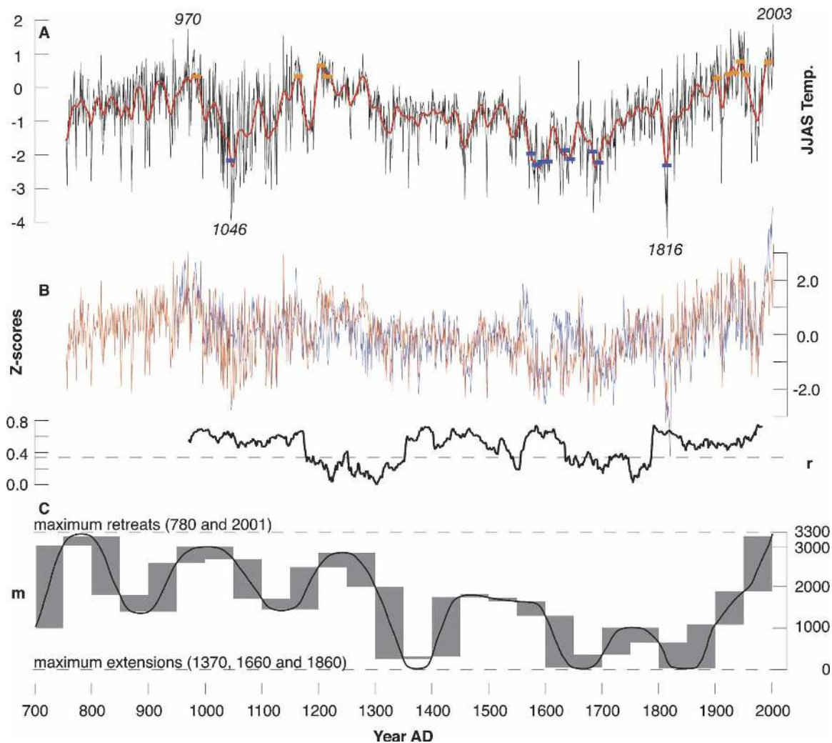
FIG. 6. (a) Alpine summer temperature reconstruction with the orange and blue boxes denoting the 10 warmest and coldest decades, respectively, and the smoothed red line being a 20-yr low-pass filter. Temperatures are expressed as anomalies w.r.t. 1901–2000. (b) High-frequency comparison between the MXD (red; this study) and RW (blue; Büntgen et al. 2005a) RCS chronologies. Records were normalized over the 951–2002 common period. The 51-yr moving correlations (black) indicate their temporal relationship, with the horizontal line denoting the 95% significance level, corrected for lag-1 autocorrelation (Trenberth 1984). (c) Length fluctuation (m) and 50-yr average mass balance (gray) of the Great Aletsch glacier (Haeberli and Holzhauser 2003).
