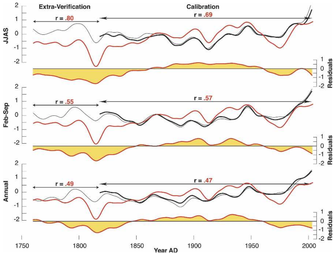
FIG. 4. Calibration (1818–2003) and extra verification (1760–1817) of the MXD–RCS chronology (red) against high-elevation (black) and low-elevation (thin) temperatures of different target season windows, using simple scaling. Residuals between 20-yr smoothed predictor and predictand indicate their relationship through time, and target season dependence. Correlations refer to unsmoothed series. Temperatures are expressed as anomalies from the twentieth-century mean.
