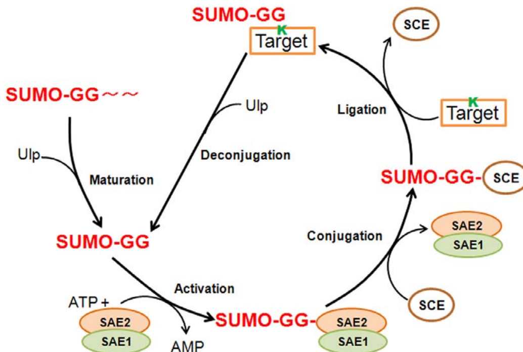
Fig. 1. The sumoylation/desumoylation cycle; Maturation, SUMO isoforms are encoded as precursor proteins and are processed by SUMO-specific cysteine proteases (ULP, ubiquitin-like protein-specific protease) with SUMO peptidase activity. Maturation consists of carboxyl terminal truncation to expose the di-glycine (GG) motif; Activation by E1, the SUMO carboxyl-terminal glycine is linked to AMP (SUMO-AMP) catalyzed by the heterodimeric E1 SUMO-activating enzymes 1 and 2 (SAE1 and SAE2) in an ATP-dependent reaction. Subsequently, the glycine of SUMO is coupled to a cysteine (C) residue in SAE2 via a high-energy thioester bond; Conjugation by E2, SUMO is transferred to a cysteine residue of the E2 SUMO-conjugating enzyme (SCE1) by transesterification catalyzed by SCE1; Ligation by E3, SUMO is transferred to the \epsilon -amino group of a lysine (K) side chain in the sumoylation consensus motif ( \psi XKE/D. \psi , a large hydrophobic residue; X, any amino acid; E/D, glutamic acid or aspartic acid) of the substrate protein, forming an isopeptide bond between the carboxyl of glycine in SUMO and the \epsilon -amino of lysine in the substrate, a process that requires the E3 SUMO ligase in vivo ; Deconjugation, SUMO-specific proteases (ULP) with isopeptidase activity cleave the isopeptide bond and SUMO is recycled through the conjugation system.
