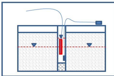
Fig. 2. Slug test with transducer and data logger.
