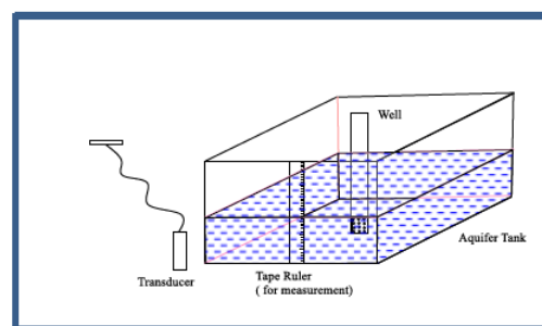
Fig. 1. Experiment tank for slug test at laboratory.
