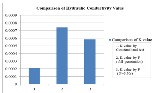
Fig. 3. Hydraulic conductivity value by Sunjoto equation (in m/sec).
