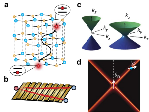
Figure 1 | Overview of super-Coulombic interaction. The proposed long-range super-Coulombic DDI may be observed ( a ) between single-photon defect centres in natural hyperbolic media (for example, h-BN, Bi 2 Se 3 and Bi 2 Te 3 ) or ( b ) between ultra-cold atoms trapped above a hyperbolic metasurface. ( c,d ) The super-Coulombic interaction occurs over a broad range of frequencies along the resonance angle of a hyperbolic medium and causes the effective interaction distance to approach zero irrespective of the physical distance.
