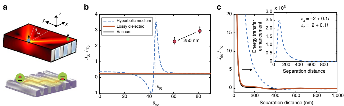
Figure 6 | Super-Coulombic CLS above hyperbolic meta-surface. CLS, J_{dd} , above hyperbolic metasurface with optic axis in the \hat{x} direction, calculated via dyadic Green function approach. Atom A and atom B are 2 nm above the interface. (a) Two-dimensional resonance cone on hyperbolic metasurfaces which causes giant in-plane long-range DDI (b) CLS dependence on angle \theta_{xy} of atom B for a fixed separation distance of r = \lambda/2 = 250 nm. The clear enhancement of the RDDI near the resonance angle \theta_R is worth noting. (c) Separation distance dependence of CLS along the resonance angle \theta_{xy} = \theta_R . Inset shows giant FRET enhancement ( > 2,000 ) for separation distances of 100 nm in the metasurface plane.
