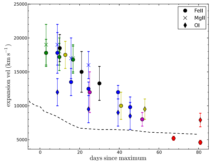
Figure 11. Expansion, photospheric velocity as measured from the different lines. Phases are relative to light curve peak. Measurements of PTF11rks (green), SN 2011ke (blue), SN 2012il (gold), PTF10hgi (red), and SN 2011kf (purple) are reported with those of SN 2010gx (black). The dashed black line shows the Fe II evolution in the normal Type Ic SN 2007gr.
