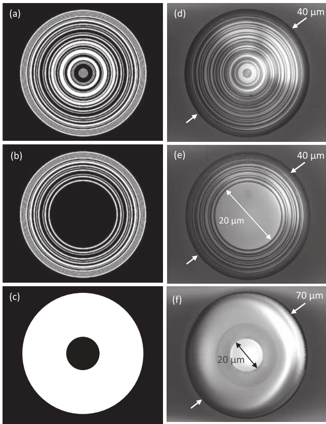
FIG. 2. Designs ((a)–(c)) and SEM images ((d)–(f)) of the of the lenses. (a) and (d) SOL, (b) and (e) ONSOL with 20 μm diameter opaque region, (c) and (f) control sample; 20 μm diameter Au disk in a 70 μm diameter transparent region.
