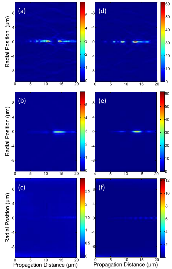
FIG. 3. Experimental ((a)–(c)) and simulated ((d) and (e)) intensity of the lens interference patterns. (a) and (d) SOL, (b) and (e) ONSOL with 20 μm diameter opaque region, (c) and (f) disc control sample. The colour scale in plots (c) and (f) has been adjusted to improve the visibility of the very low intensity spots.
