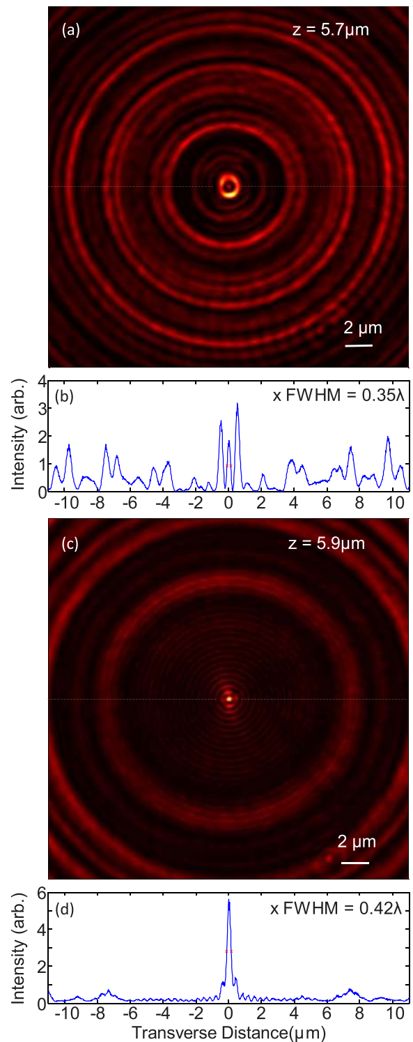
FIG. 5. Focal spots at (a) z = 5.7\ \mu\text{m} for the SOL and at (c) z = 5.9\ \mu\text{m} for the ONSOL. (b) and (d) show intensity profiles through the lines in (a) and (c), respectively.
