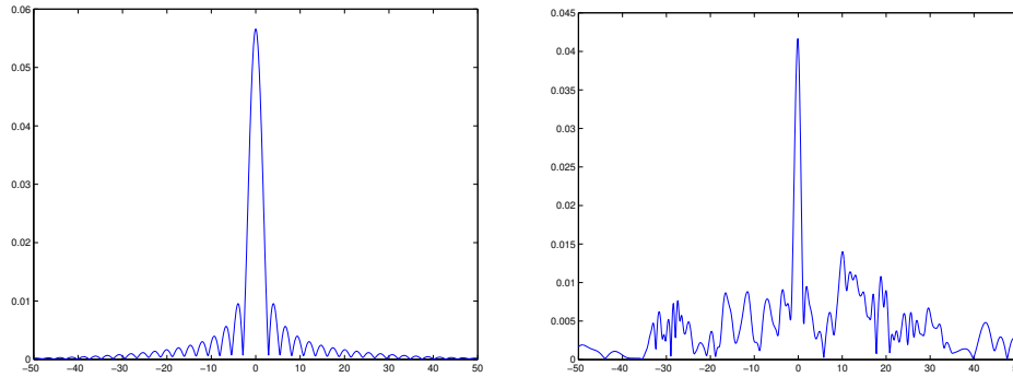
Figure 13: The re-compressed pulse for homogeneous (left) and random (right) media. The propagation distance is 800m, the domain width is 100m, and the maximal contrast is 10%. The boundary conditions are: DTBC . TRM width 100m. Here, we can see clearly super-resolution as the re-compressed peak is narrower in the random medium.
