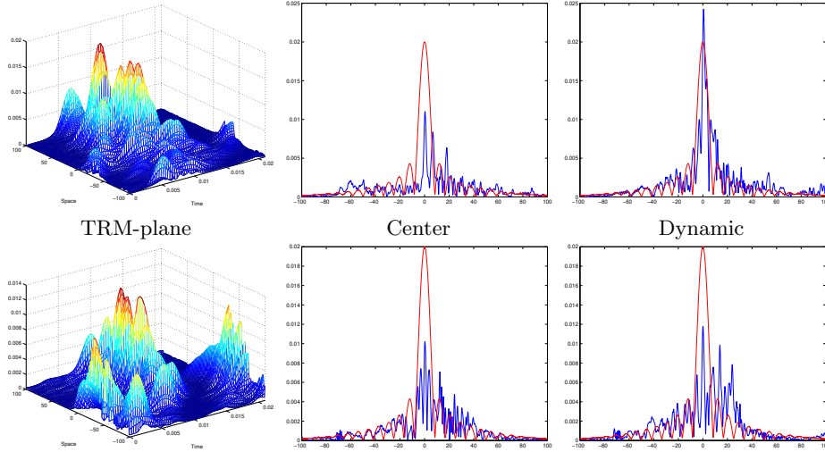
Figure 12: Dynamic TRM placement: 1000m propagation. (For parameter information see the caption for figure 11).
