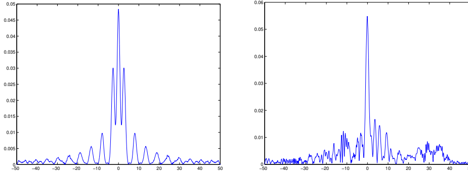
Figure 17: Homogeneous medium on the left, random medium on the right. Type of boundary conditions: Wave-Guide with TRM width 50m . The wave-guide effects are quite strong, but there is super-resolution since the peak is better defined in the random medium.
