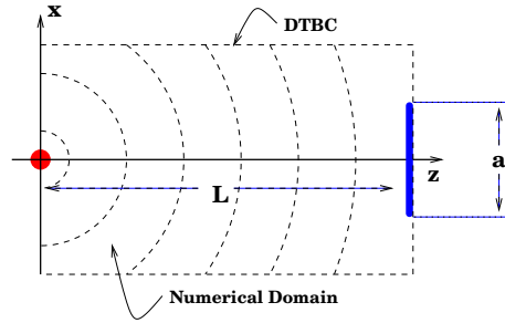
Figure 1: Setting for time-reversal acoustics. A point source (red) emits a wave, which is received on a screen (blue) of width a — the time-reversal mirror (TRM) — at a distance L from the source. The domain of numerical solution of the (parabolic) wave equation is shown with a dotted line, and DTBC stands for Discrete Transparent Boundary Conditions .
