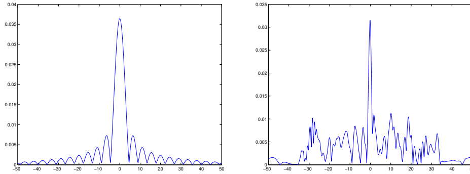
Figure 15: Homogeneous medium on the left, random medium on the right. Type of boundary conditions: DTBC with TRM width 60m . We can clearly see super-resolution as the re-compressed peak is narrower in the random medium case. The fluctuations in the side-lobes are partly due to the fact that we are pushing the paraxial approximation beyond its limit; the 10% contrast is stretching the “low-contrast” assumption.
