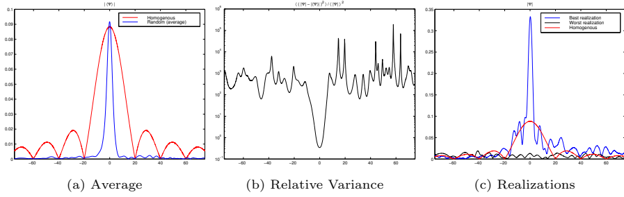
Figure 2: Time-harmonic waves in random media. Propagation distance 1000m, TRM width 50m, width of numerical domain 150m, width of random medium 112.5m, contrast \pm 5\% , 428 realizations. (a) Amplitude of the mean: Homogeneous (red) and average over random realizations (blue) case. (b) Relative variance, > \mathcal{O}(1) except for a very small interval. (c) Individual realizations that show super-resolution (blue) as well as no resolution at all (black).
