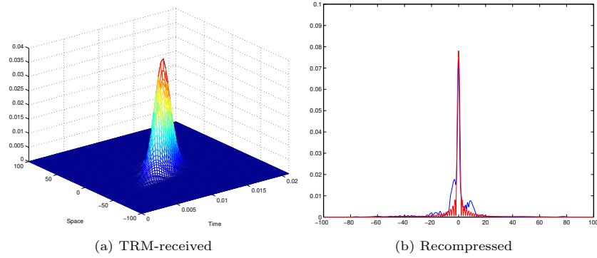
Figure 7: Numerical simulation of time-reversal. The width of the time reversal mirror and the numerical domain are 50m, and 200m, respectively. The maximum contrast is \pm 10\% , that is |\mu| \leq 0.1 . The left figure shows the signal as received on the TRM-plane. This signal is restricted to the mirror, time-reversed, and re-emitted into the medium. The right figure shows a spatial section through the re-focussed signal. Here, the propagation distance is very short, only 200m, or about 20 correlation lengths. We see that there is not enough randomness to observe super-resolution.
