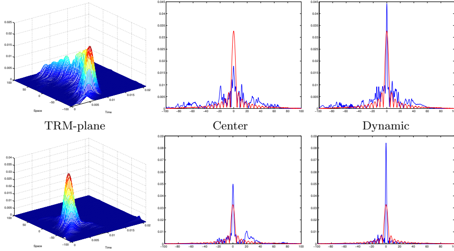
Figure 11: Dynamic TRM placement: 600m propagation. THE LEFT FIGURE shows the pulse in space-time as received on the TRM-plane. THE CENTER FIGURE shows a spatial cut through the peak of the re-compressed pulse using static TRM placement. THE RIGHT FIGURE shows a spatial cut through the peak of the re-compressed pulse using optimal dynamic TRM placement. Note that each plot is for one random realization of the medium. The maximum contrast is 10%, that is |\mu| \leq 0.1 . The TRM is 50 meters wide and the numerical domain 200 meters wide. The red curves correspond to time-reversal in a homogeneous medium and the blue curves to time-reversal in the random medium.
