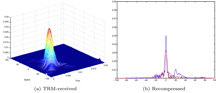
Figure 8: In this simulation the propagation distance is 600m. Now we clearly see the super-resolution phenomenon: the peak of the re-compressed pulse in the random medium (blue) is sharper than the one for the homogeneous medium (red). (All other parameters are as in figure 7.)
