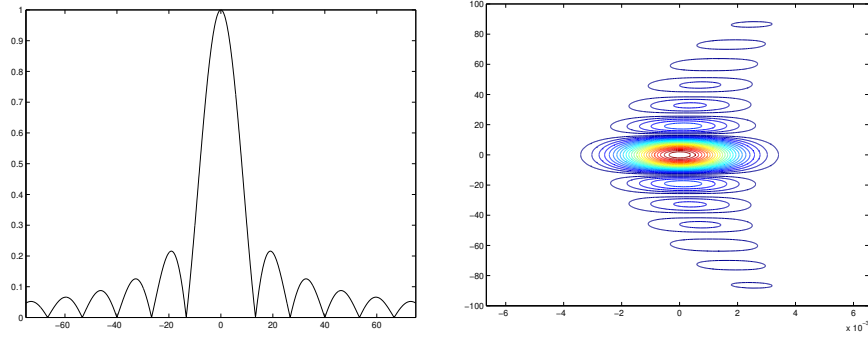
Figure 3: The left figure shows the spatial diffraction pattern of the amplitude of (25) at time t = 0 . The right figure is a space-time contour plot of the amplitude of (25) and shows the parabolic shift in arrival time. Here the pulse width is \sigma_t = 1.33\text{ms} , the TRM width a = 50\text{m} , the propagation speed is c_0 = 1500\text{m/s} , the propagation distance is L = 1000\text{m} , and the period of the carrier is 0.22\text{ms} at 4.5\text{KHz} .
