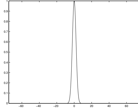
Figure 4: The spatial shape of the compressed pulse with a Gaussian aperture function at time t = 0 , from (31). Here the pulse width is \sigma_t = 1.33\text{ms} , the TRM width is a = 50\text{m} , the propagation speed is c = 1500\text{m/s} , propagation distance is L = 1000\text{m} , and the time period of the carrier is 0.22\text{ms} . Note the absence of Fresnel zones for a Gaussian TRM.
