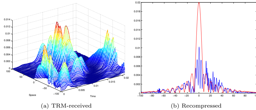
Figure 9: In this simulation the propagation distance is 1000m. Although the first peak of the recompressed signal in the random medium is much narrower, there is really no super-resolution in this case because of the large side-lobes. The limits of the numerical simulations are discussed in section 8.2. (All other parameters as in figure 7.)
