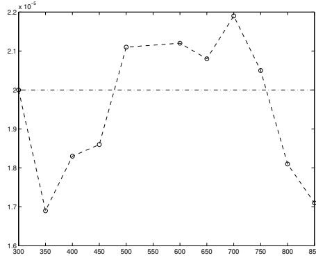
Figure 10: The estimated values of \gamma for table 1. The estimate stabilizes as the propagation distance increases, until the numerical setup cannot capture adequately the multipathing and the rapidly growing effective aperture. In our setup we can simulate an effective aperture up to about twice the width of the random medium.
