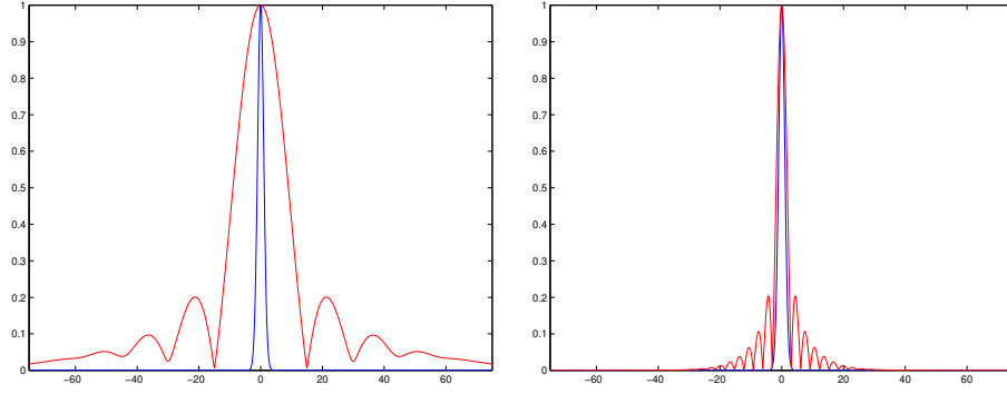
Figure 5: Comparison of the theoretical formula (56) at time t = 0 , for a medium with L = 600m , a_e = 195m , \gamma = 2.12 \times 10^{-5} m^{-1} . THE LEFT FIGURE shows a plot of (56) for a homogeneous medium, \gamma = 0 , with a TRM of width a = 40 (in red / wide Fresnel zone), and the random medium with \gamma = 2.12 \times 10^{-5} and a = 40 (in blue / narrow Fresnel zone). THE RIGHT FIGURE shows a plot of (56) for a homogeneous medium, \gamma = 0 , with a = a_e = 195 (in red), and the random medium with \gamma = 2.12 \times 10^{-5} , and a = 40 (in blue). The match confirms the validity of (57). The values of a_e and \gamma originate from the numerical estimates of the effective aperture summarized in table 1 in section 8.
