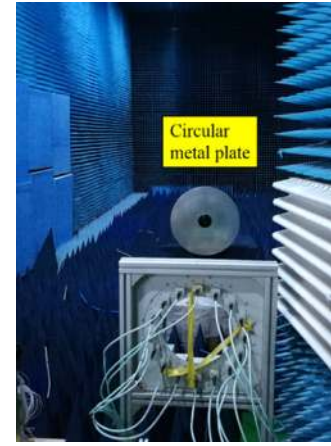
FIG. 8. Photograph of imaging scenario of the circular metal plate.
