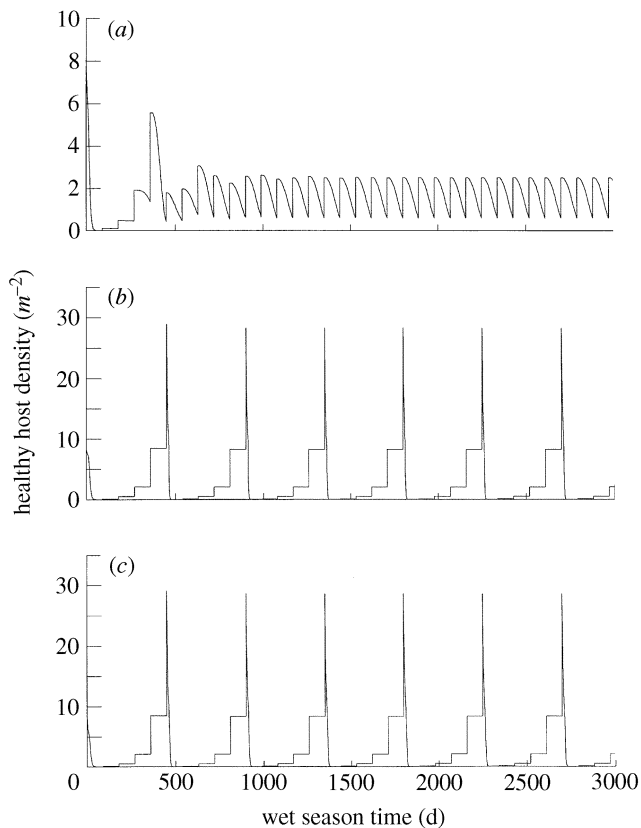
Figure 2. Dynamics implied by the best fit parameter sets for each alternative model. These dynamics are qualitatively similar to those observed in every bootstrap replicate run for their respective models. The vertical axes are healthy host densities ( m^{-2} ). The time axes are days within wet seasons: discontinuities occur for between-season dynamics. It is assumed that host densities above 10 m^{-2} trigger spraying, with an initial contact rate of 15% and a decay in residual infectivity as measured in Thomas et al. (1997). (a) Hochberg's (1991) model predicts sustained control with a single pathogen application in the first season. (b) The Briggs & Godfray (1995) model predicts that pathogen must be applied every six years. (c) The Michaelis-Menten model makes almost identical predictions to the Briggs & Godfray (1995) model. Note the change in vertical scale between (a) and the other plots. We also ran stochastic simulations in which the transmission model parameters were reset at the beginning of each rainy season by sampling from the population of parameter sets obtained by bootstrapping: the qualitative results were unchanged. Hochberg's (1991) model gives sustained control after a single application of pathogen, while the other two models require regular and frequent spraying to prevent population explosions.
