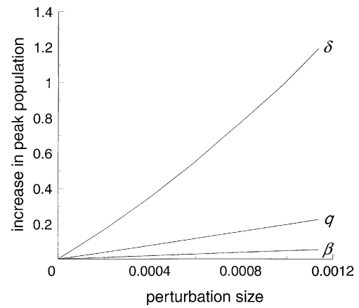
Figure 5. Relative sensitivity of predictions of the model of §2 to perturbations of equal magnitude, produced by different parameters. The vertical axis is the predicted increase in peak host population. The horizontal axis is the magnitude of the perturbation as measured by the metric d given in §3. These perturbations were produced by variation of \delta , \beta and q , so each perturbation represents a different direction in the space of functions used in the model. Perturbations of \beta and q restrict variation to the manifold of the Hochberg (1991) model, while perturbation of \delta causes variation off that manifold. Clearly predictions are much more sensitive to \delta than to the other parameters.
