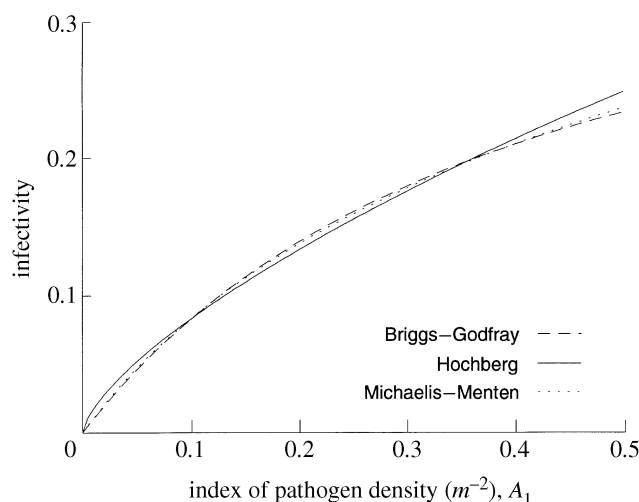
Figure 1. Comparison of the shapes of the best fitting nonlinear transmission models, over the range of pathogen density index present in the experiment (the Hochberg (1991) model pathogen density index range was 0–0.3; other models went as high as 0.8 for short periods—although one can repeat the entire analysis presented in this paper with lower spray action thresholds to bring this figure below 0.5: conclusions are unaltered). The index of pathogen density is the quantity A_1 in the model equations and is proportional to the density of fungal spores ( m^{-2} ). See table 1 for model descriptions and parameter values. Infectivity is an individual's instantaneous daily infection risk.
