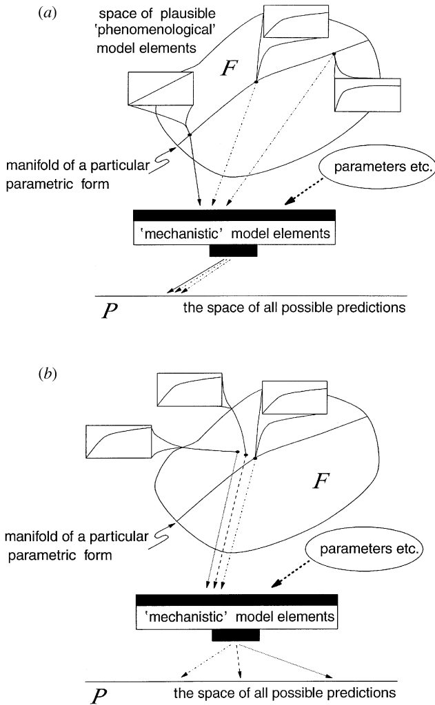
Figure 4. Approximate schematic representation of how super-sensitivity to structure is generated. The mechanistic elements of a model can be thought of as a way of combining phenomenological model elements and other model inputs to produce predictions. In the diagrams the space F of all plausible phenomenological elements is a space of one-dimensional functions—each ‘point’ in this space is one such function (a functional form and parameter values). The panels show functions that are five elements of the space. The arrows illustrate how incorporating a particular function from F into the model generates a particular prediction, with the type of dashing on the arrows indicating which function gives which prediction. In general, the change in predictions made by the model as we move within F will depend not only on how far we move, but also in which direction. (a) How substantial movement in F along the path generated by varying the parameters of a particular functional form might make little difference to predictions. (b) A contrasting scenario in which comparatively small movements within F , off the manifold of the particular functional form, produce large changes in predictions.
