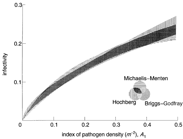
Figure 3. The 98% confidence bands obtained by parametric bootstrapping for the three models. The level and type of shading indicates the three bands and the regions of overlap of the different bands. (It may be helpful when viewing this figure to imagine that the bands are made of light-polarizing material whose polarization direction is given by the directions of the shading lines.)
