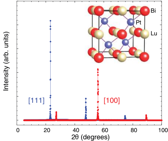
FIG. 1. (Color online) X-ray diffraction data along the [100] (red) and [111] (blue) crystallographic directions. The interplanar distance along the [111] direction is 3.801 Å, consistent with the cubic lattice parameter a = 6.578 Å. Inset: the conventional unit cell of LuPtBi. This noncentrosymmetric structure, common to all the XYZ half-Heusler family, belongs to the F\bar{4}3m space group. By taking out the X atom (Lu in this case), we obtain the zinc-blend structure of the HgTe.
