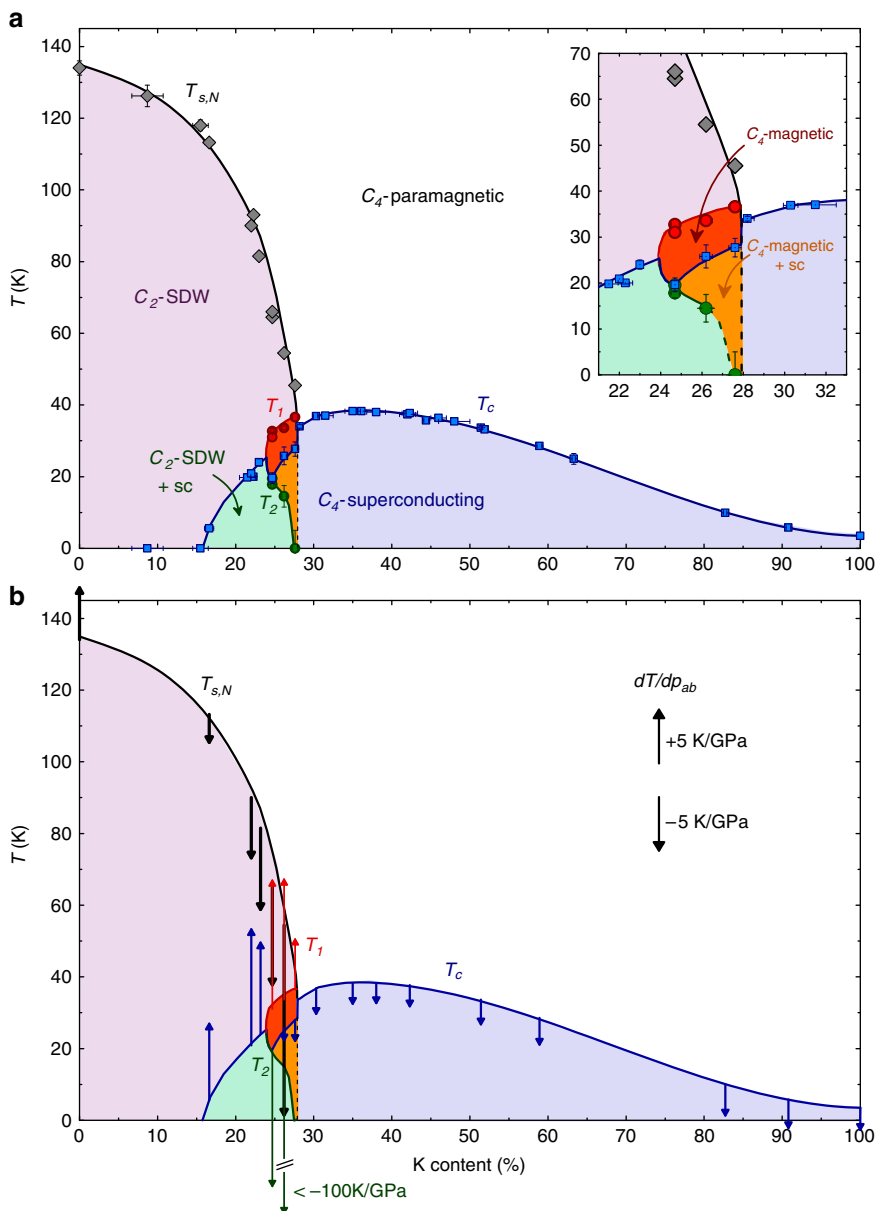
Figure 3 | Detailed phase diagram of \text{Ba}_{1-x}\text{K}_x\text{Fe}_2\text{As}_2 . (a) Phase diagram of \text{Ba}_{1-x}\text{K}_x\text{Fe}_2\text{As}_2 spanning the whole substitution range. T_{s,N} , T_1 , T_2 and T_c (determined from the data shown in Fig. 2 and additional thermodynamic data) are shown by symbols. Lines and coloured areas are a guide to the eye indicating the five distinct thermodynamically ordered phases. A narrow region of a C_4 -symmetric (tetragonal) magnetic phase, occurring within the usual C_2 -symmetric (orthorhombic) SDW phase, is observed. It coexists with superconductivity with a reduced T_c . Superconductivity-induced reentrance of the C_2 -SDW phase occurs at T_2 . The inset shows an enlarged view of the region containing the C_4 -magnetic phase. Vertical error bars indicate the uncertainty in the transition temperatures and horizontal error bars indicate the statistical error in the sample composition. (b) Predicted effect of uniaxial in-plane pressure p_{ab} on the phase diagram, from thermodynamic relations using our thermal-expansion and heat-capacity data. The direction of the arrows indicates the sign of the pressure derivative of the transition temperature and the length is proportional to its absolute value (see scale). Lines are reproduced from panel (a).
