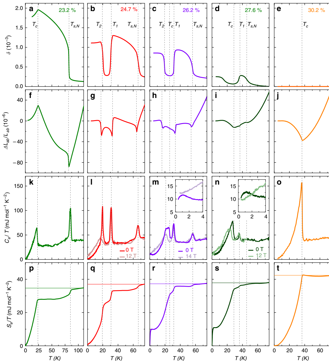
Figure 2 | Phase transitions in thermal expansion and electronic specific heat for 5 samples of different K content. (a–e) Orthorhombic distortion \delta , (f–j) average in-plane length change \Delta L_{ab}/L_{ab} for ‘twinned’ samples (k–o) electronic specific heat C_e/T , (p–t) electronic entropy divided by temperature S_e/T . Horizontal lines indicate the value of S_e/T of the high-temperature paramagnetic phase which is lost on cooling through the various transitions. (l–n) also show data measured in a large magnetic field and the insets show a magnification of the low-temperature region. Vertical lines mark the transitions temperatures labelled in panels (a–e).
