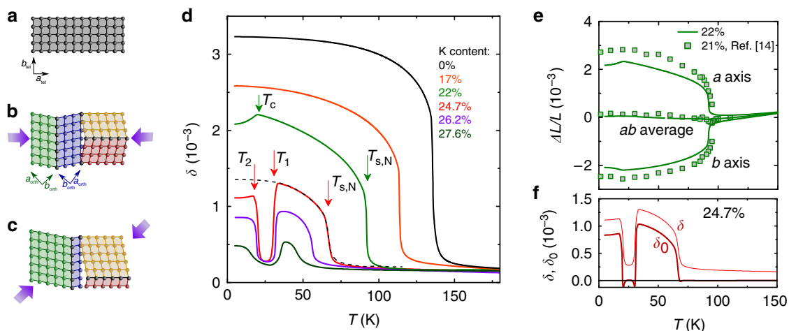
Figure 1 | Orthorhombic distortion of \text{Ba}_{1-x}\text{K}_x\text{Fe}_2\text{As}_2 as measured using a capacitance dilatometer. (a) Schematic representation of the tetragonal C_4 high-temperature phase. (b) Representation of the structural domains formed in the orthorhombic C_2 phase ('twins', indicated by different colours). The domain structure is unaffected by the force from the spring-loaded dilatometer if it is applied along the tetragonal [100] in-plane direction (purple arrows). (c) Representation of the mostly 'detwinned' state, achieved by applying the dilatometer force along [110], which selects the domains with their (shorter) orthorhombic b axis along the direction of the applied force. (d) Temperature dependence of the orthorhombic distortion \delta = (a - b)/(a + b) of underdoped \text{Ba}_{1-x}\text{K}_x\text{Fe}_2\text{As}_2 obtained using difference of 'twinned' and 'detwinned' data from our high-resolution capacitance dilatometer. Abrupt changes of \delta mark phase transitions, examples of which are indicated by vertical arrows. (e) Good agreement between our results (continuous lines), and results from neutron powder diffraction 14 (symbols) for the thermal expansion of the a and b axis demonstrates the reliability of our technique. (f) Orthorhombic distortion corrected for the effect of the applied force, \delta_0 , for the sample with 24.7% K content, distinguishing tetragonal and orthorhombic phases (see Supplementary Figs 1 and 2 for details on the measurement of the orthorhombic distortion).
