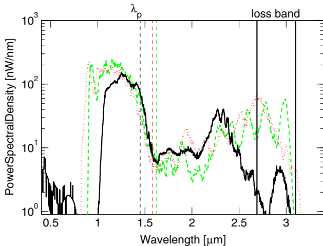
Fig. 7. (Color online) Measurement (black) and simulations (dashed green) of SCG for \lambda_p = 1450 \text{ nm} and P_0 = 710 \text{ kW} . The dotted red spectrum is obtained for the wavelength-shifted dispersion profile in Fig. 2]. Dashed vertical lines mark pump wavelength (black) and the ZDW (red, green) of the fiber.
