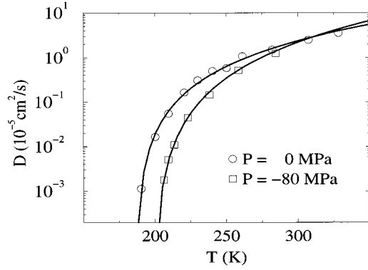
FIG. 10. Temperature dependence of the diffusion coefficient D for two isobars. \square are from Table I and \circ from [30]. Full lines are power-law fits, respectively, given by D=13.93(T/198.7-1)^{2.73} and D=7.39(T/186.3-1)^{2.29} , where D is in \text{cm}^2/\text{s} and T is in K.
