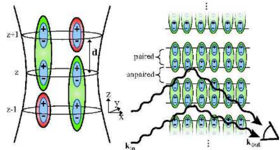
FIG. 1. Schematic representation of competition for pairing among adjacent pairs of layers, including depiction of the optical confinement beam which creates the stack of 2D sheets (left), and illustration of one of the two equivalent dimerized pairing ground states for a many layered system (right). The wavy lines illustrate the proposed light-scattering detection scheme discussed below in the text.
