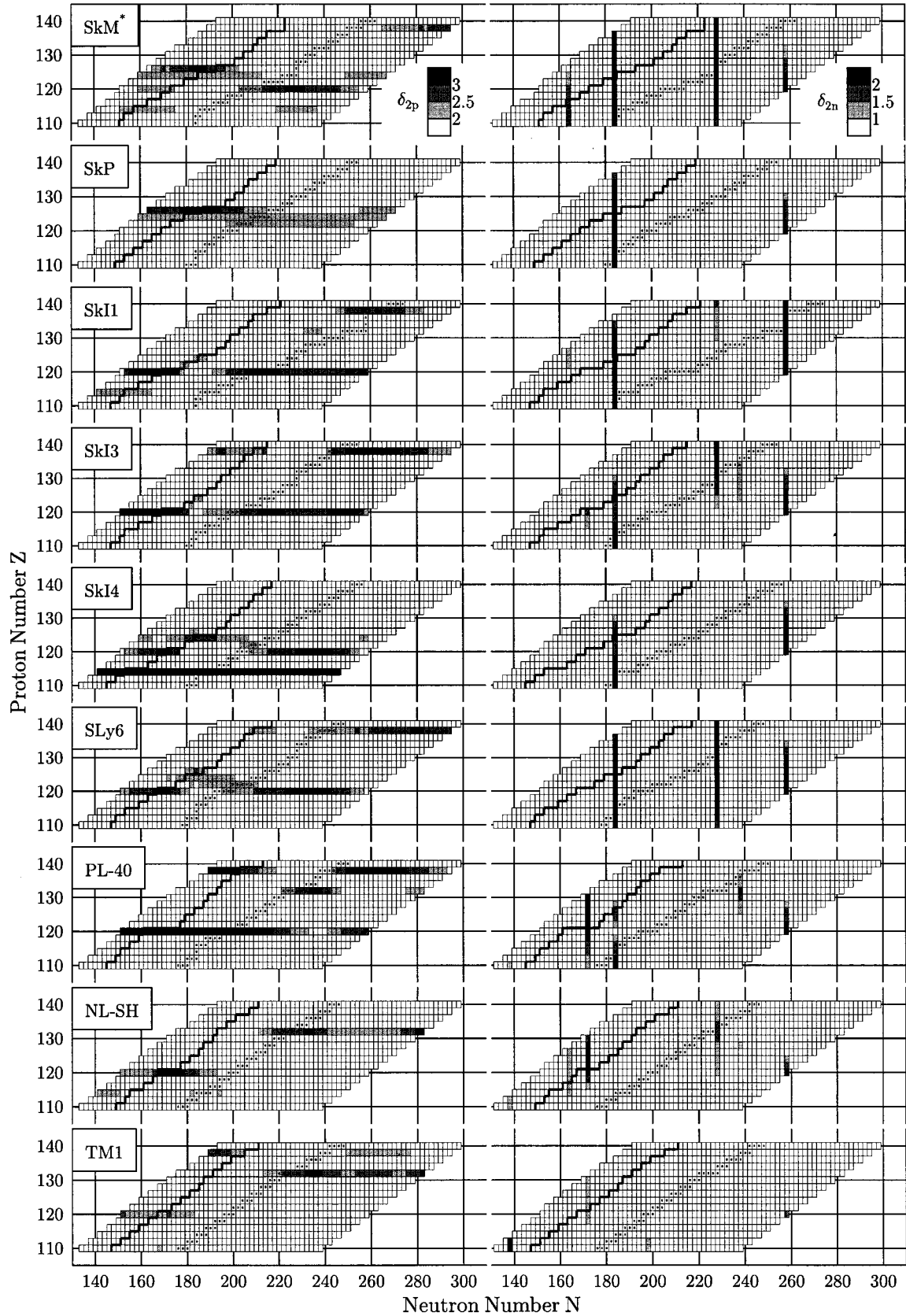
FIG. 1. Grey scale plots of proton gaps (left column) and neutron gaps (right column) in the N - Z plane for spherical calculations with the forces as indicated. The assignment of scales differs for protons and neutrons, see the uppermost boxes where the scales are indicated in units of MeV. Nuclei that are stable with respect to \beta decay and the two-proton dripline are emphasized.
