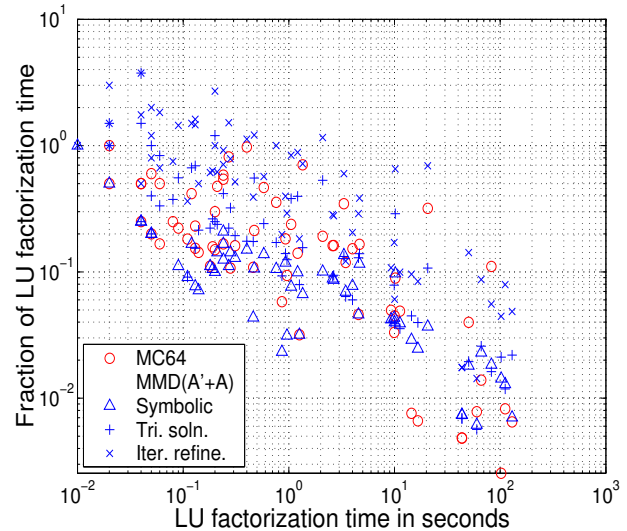
Figure 7: The times for the other steps of GESP, as fraction of the factorization time.
