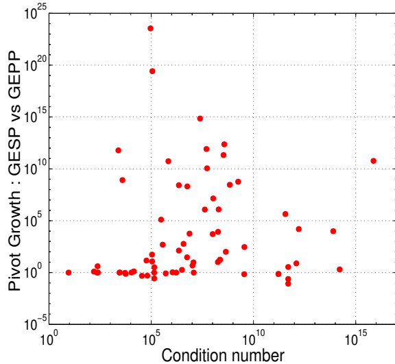
Figure 6: The ratio of pivot growth of GESP versus GEPP.
