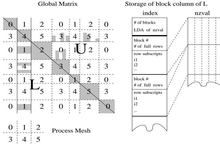
Figure 9: The 2D block-cyclic layout and the data structure to store a local block column of L .
