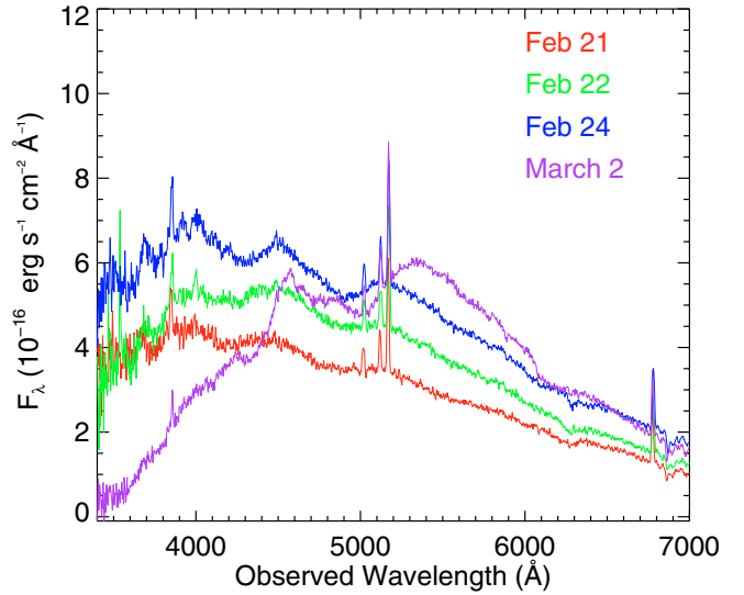
Fig. 2. The flux-calibrated and de-reddened spectra of the emerging supernova. The spectra have been absolute flux-calibrated by comparison to V -band photometry. In the Feb. 24 spectrum we note some components of intermediate widths \sim 3000 – 4000 km s ^{-1} in the blue part of the spectrum.
