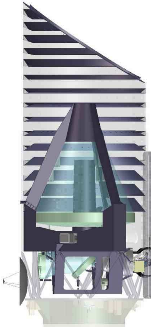
Fig. 14.— Schematic treatment of the outer baffle interior vane arrangement. Sunlight is incident from the left, where the height of the baffle and its angled forward edge maintains the baffle interior in darkness.
