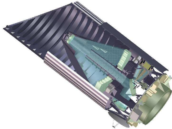
Fig. 11.— Cutaway view of the reference SNAP design. The entire telescope attaches to the spacecraft structure by means of bipods. The outer baffle, shown cut away, also attaches to the spacecraft structure by means of its separate supporting struts. A discardable door, shown open in light gray, protects the cleanliness of the optics until on-orbit commissioning begins. Solar panels are fixed, not deployed.
