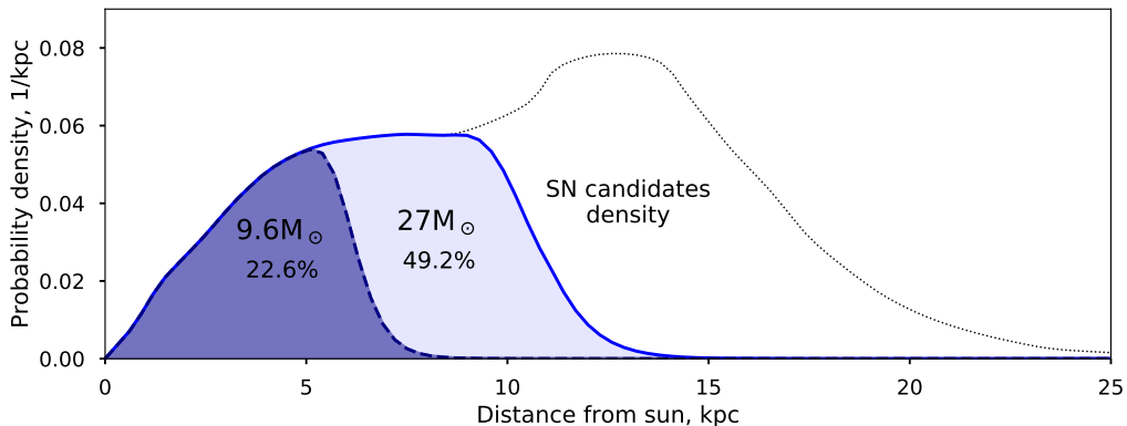
Figure 15. The NOvA experiment’s sensitivity to galactic supernova vs. distance. The dark blue area is for a 9.6M_{\odot} progenitor, and the light blue area from a brighter 27M_{\odot} star: both models are from [13]. The dotted curve for supernova progenitor density is from [27]. Percentage is the fraction of SN candidates covered by the trigger, for the two cases of progenitor masses.
