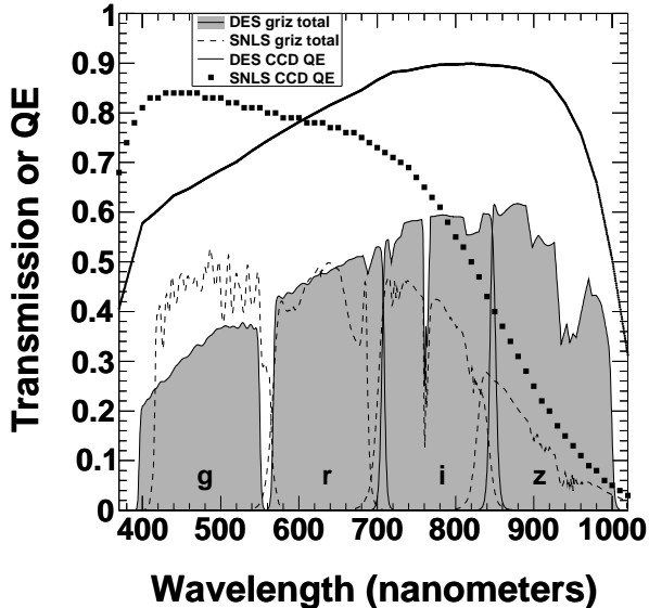
Fig. 2.— Comparison of the SNLS (Regnault et al. 2009) and DECam total transmission (H. Lin, private communication, 2011) for an airmass of 1.3. Also shown is the CCD quantum efficiency (QE). The total transmission includes the effects of QE, the atmosphere, and the optical systems of the relevant cameras. Note the increased DES sensitivity at redder wavelengths. The DECam transmission is based on measurements of the full-size filters, which was not available during the simulations performed for this analysis. The assumed transmission in this paper is about 10% smaller than the measured values.
