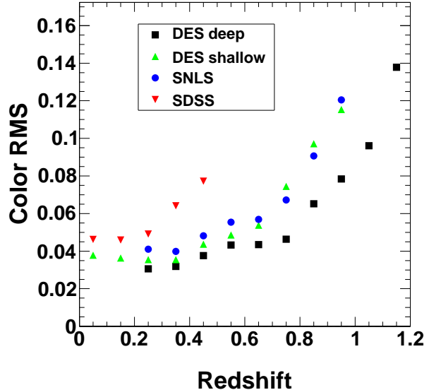
Fig. 3.— Simulation of the scatter in the SALT2 color parameter for the SDSS, SNLS, and DES supernova samples highlighting the red advantage of the DES. The simulation method and DES implementation are discussed in §2 and §3, respectively.
