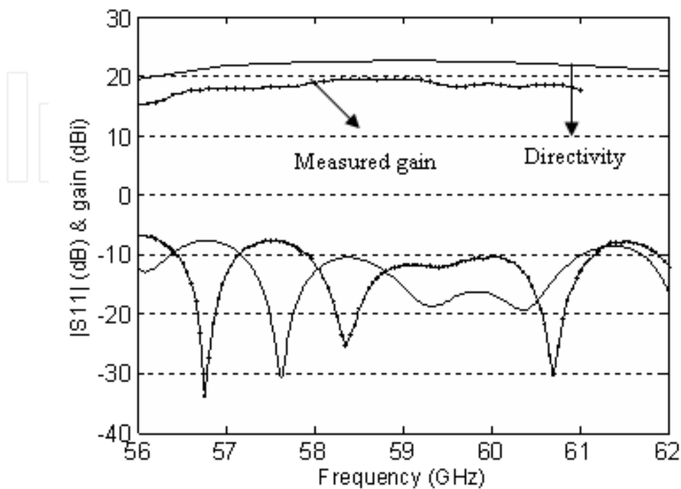
Fig. 18. Variation of S11 and gain with a square superstrate dimension of 6 \lambda_0 . Simulation ——— measured —•—.
