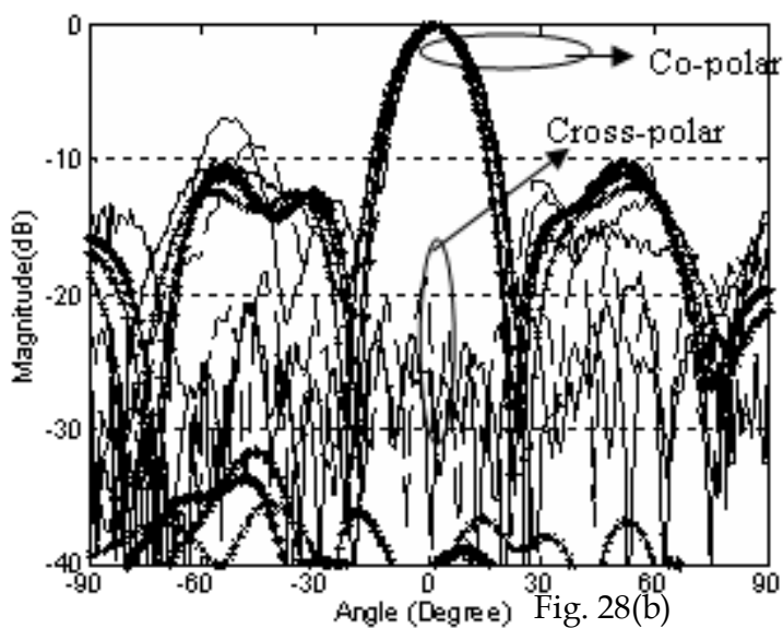
Fig. 28. Measured and simulated H-plane (a) & E-plane (b) radiation patterns of the 2 x 2 superstrate antenna array (Co and Cross polarisation).
