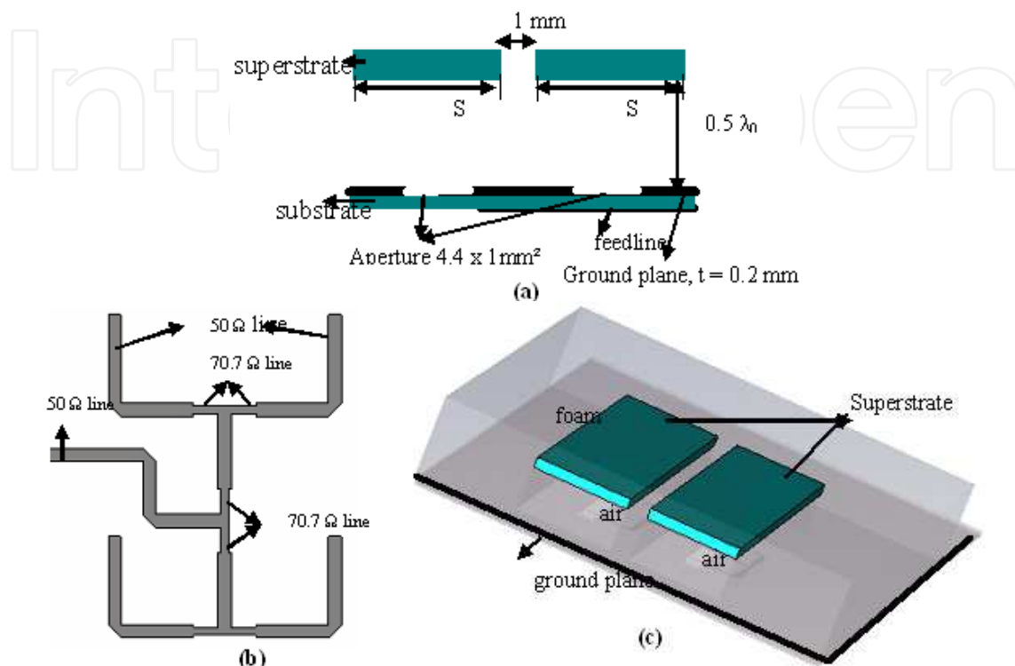
Fig. 25. (a) Cutting plane of a 2 \times 2 aperture antenna array with superstrate, ground plane size = 6 \lambda_0 \times 10 \lambda_0 for connecting V band connector and for ease of measurement purpose. (b) 2 \times 2 feed network. (c) Overview of 2 \times 2 array prototype: details of the two separate superstrate sheets and air gap within foam.
