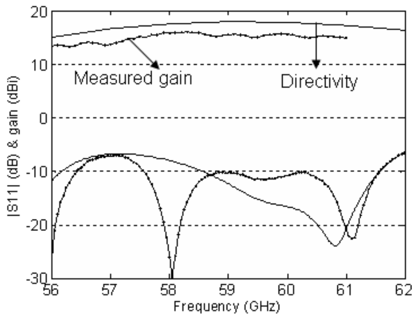
Fig. 14. Variation of S11 and gain with a superstrate dimension of 3.2 \lambda_0 . Simulation ——— measured —•— .
