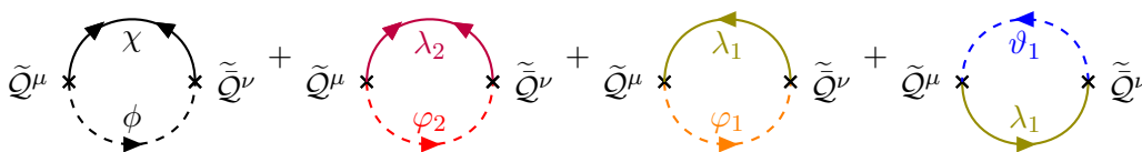
Figure 4. One-loop diagrams that contribute to the supercurrent 2-point function.
